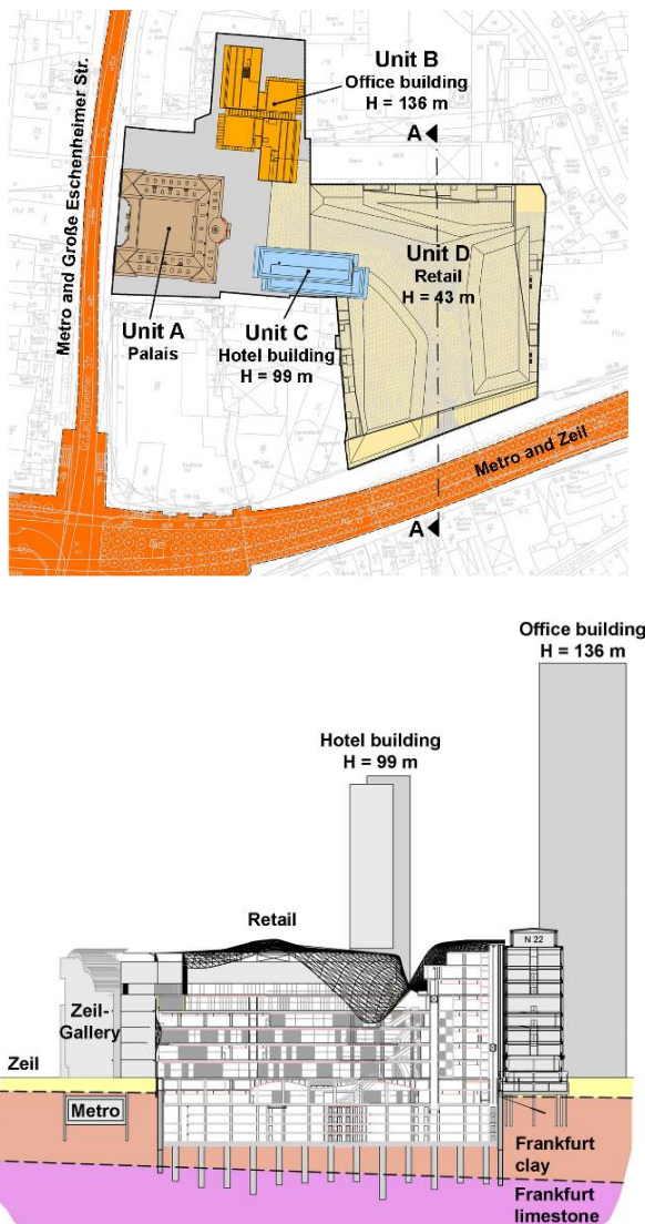
Figure 8 PalaisQuartier complex in Frankfurt am Main, Germany: plan view (top) and cross section A-A (bottom)
