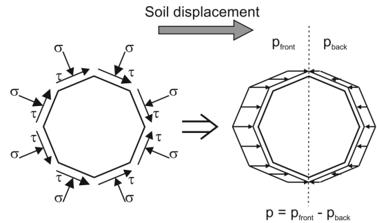
Figure 12 Lateral pressure acting on the pile derived from normal stresses and shear stresses at the pile-soil interface
