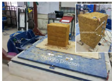
Shaking table test on soil block (After Tanaka and Lee, 2016)
