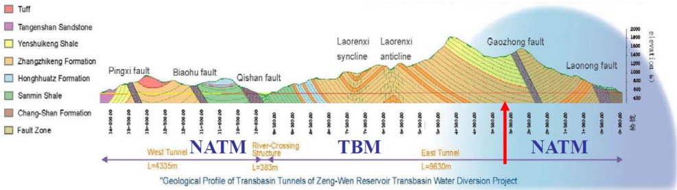
Figure 3 Geological profile along tunnels in TDT project
