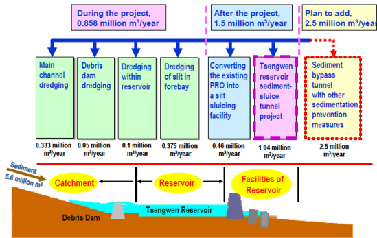
Figure 2 Master plan for sediment management at Tsengwen Reservoir
