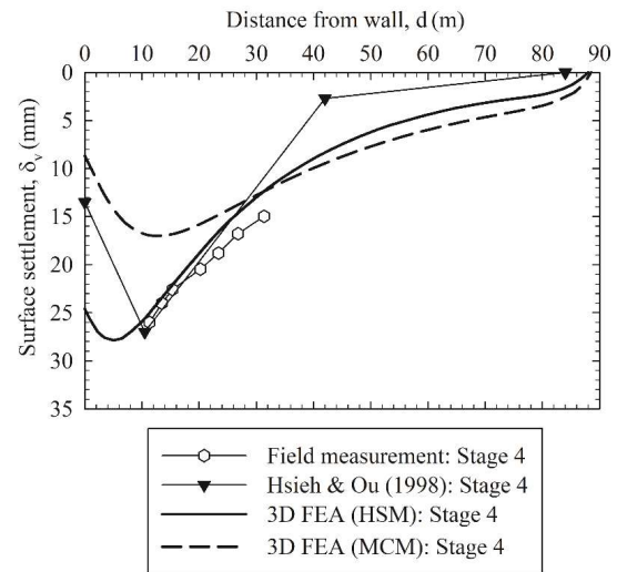
Figure 13 Comparison of ground surface settlement prediction at final stage
