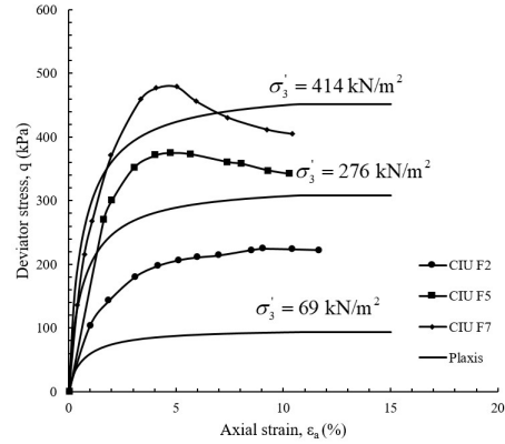
Figure 3 Hyperbolic stress-strain curves of Bangkok stiff clay
