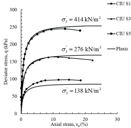
Figure 1 Hyperbolic stress-strain curves of Bangkok soft clay
