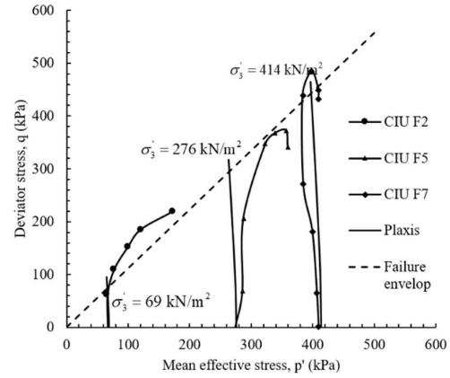
Figure 4 p'-q stress path of Bangkok stiff clay
