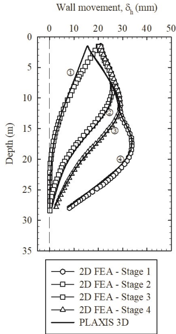
Figure 10 Comparison wall deformation between 2D FEA after Likitlersuang et al. (2013a) and 3D FEA with HSM at the middle of the long wall
