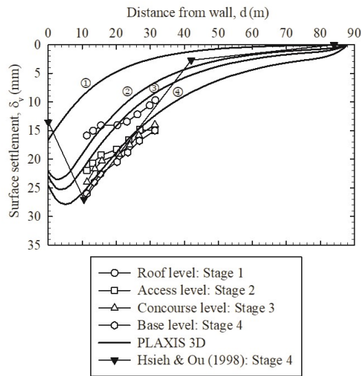
Figure 11 Comparison of ground surface settlement between 3D FEA with HSM, SS1 and empirical relationship
