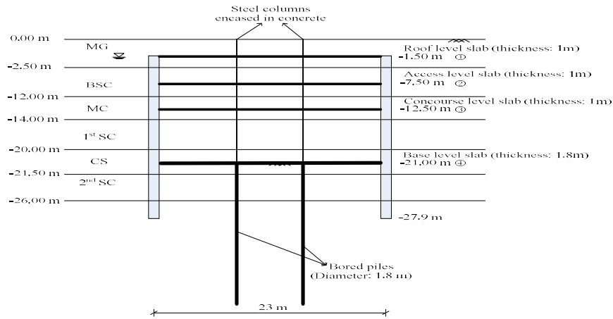
Figure 7 Cross section (AA) of Sukhumvit MRT Station
