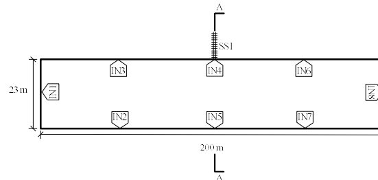
Figure 5 Sukhumvit MRT Station layout
