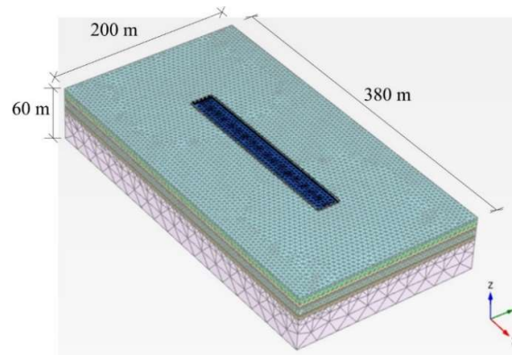
Figure 6 Finite element and mesh generation (295,081 elements and average size of 3.96m) (after, Chheng and Likitlersuang, 2018)
