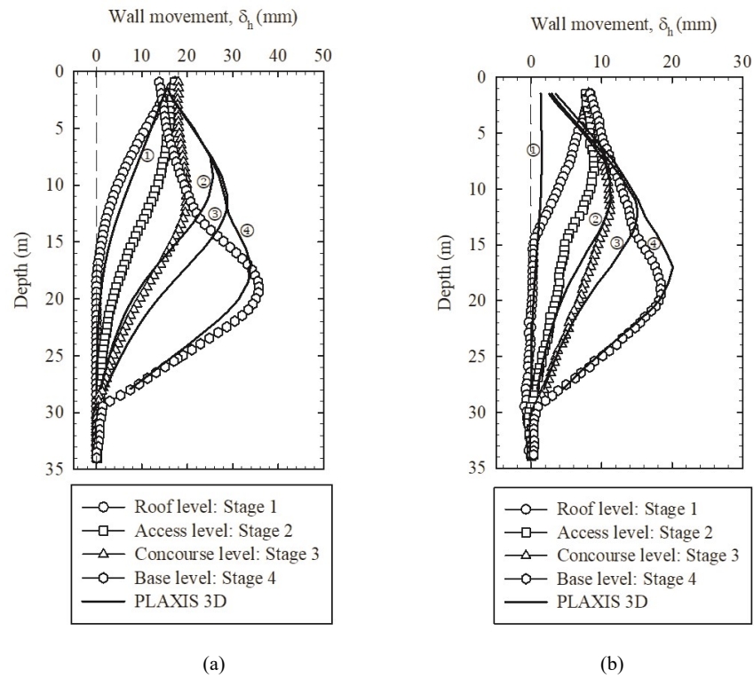
Figure 8 Comparison between 3D FEA with HSM and inclinometers: (a) IN4, (b) IN8 (after, Chheng and Likitlersuang, 2018)
