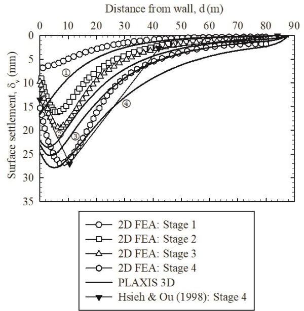
Figure 12 Comparison of ground surface settlement between 3D FEA with HSM and 2D FEA with HSM from Likitlersuang et al. (2013a)
