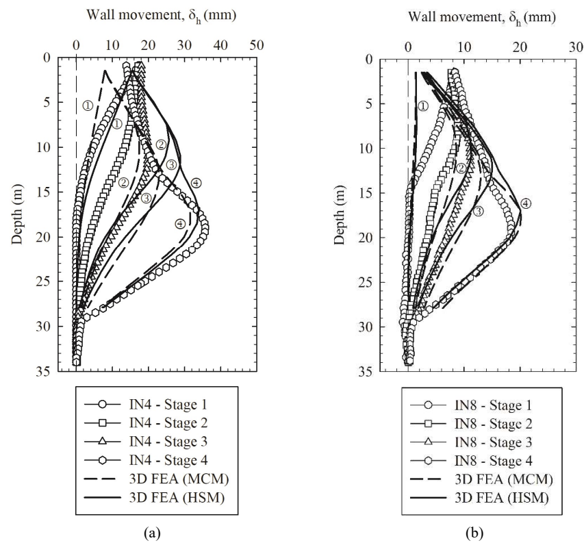
Figure 9 Wall deformation comparison between field data, MCM and HSM
