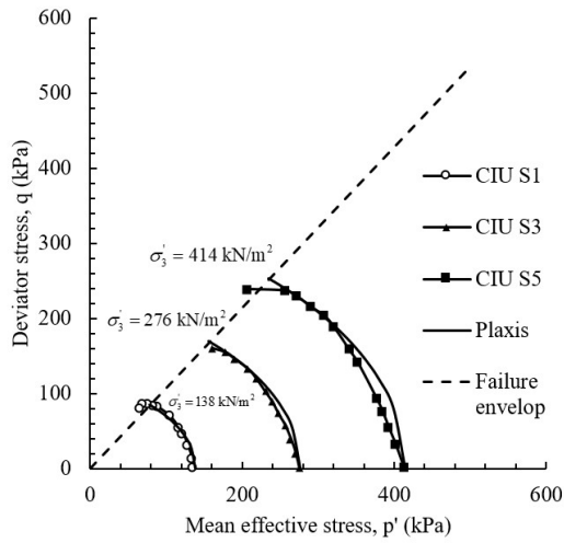
Figure 2 p'-q stress path of Bangkok soft clay
