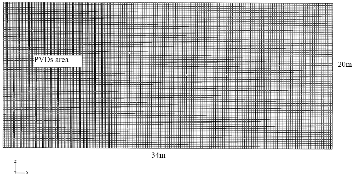
Fig. 8. 2D finite element mesh discretisation
