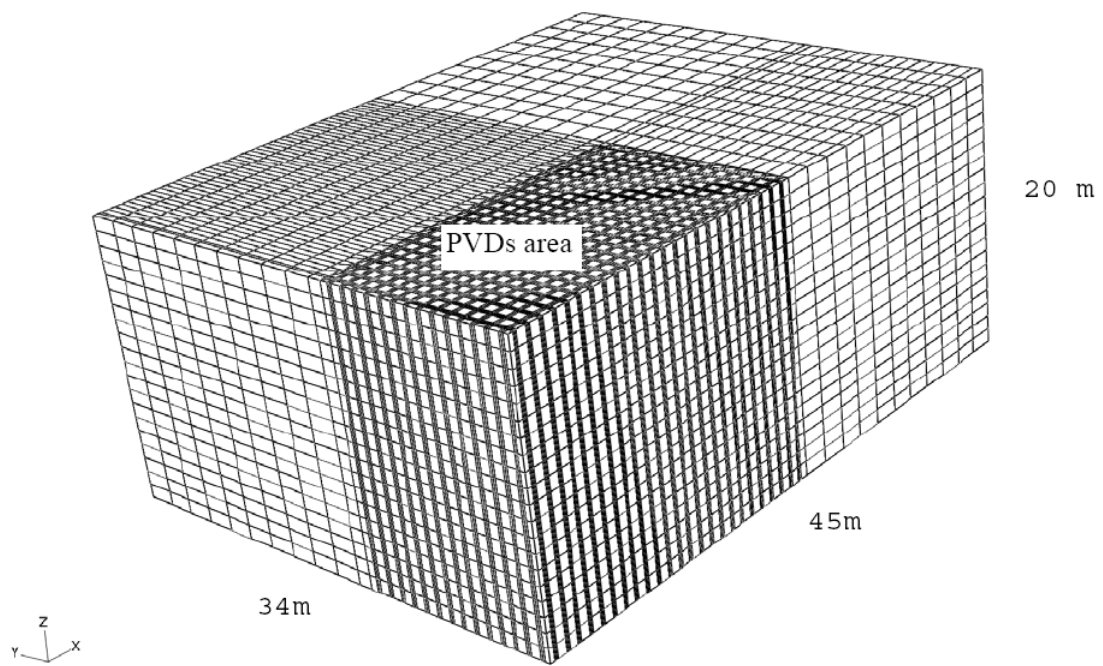
Fig. 7. 3D finite element mesh discretisation
