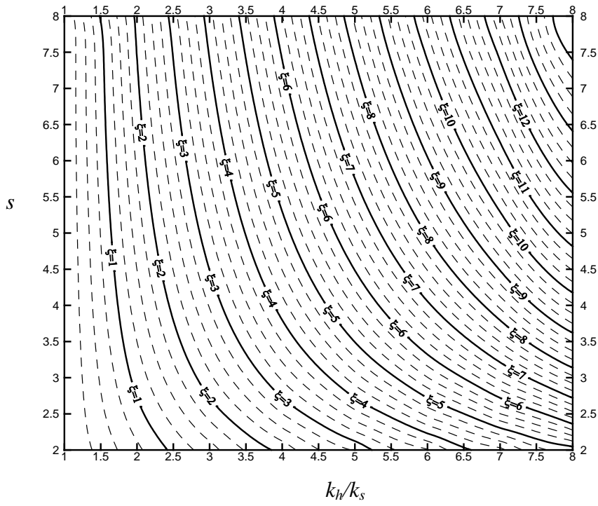
Fig. 13. Contour plot of \xi based on Equation (19) (Rujikiatkamjorn and Indraratna 2009)
