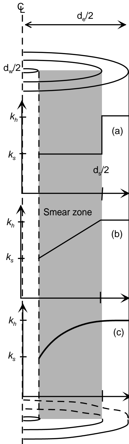
Fig. 2. Permeability distribution in smear zone (a) constant (b) linear and (c) parabolic
