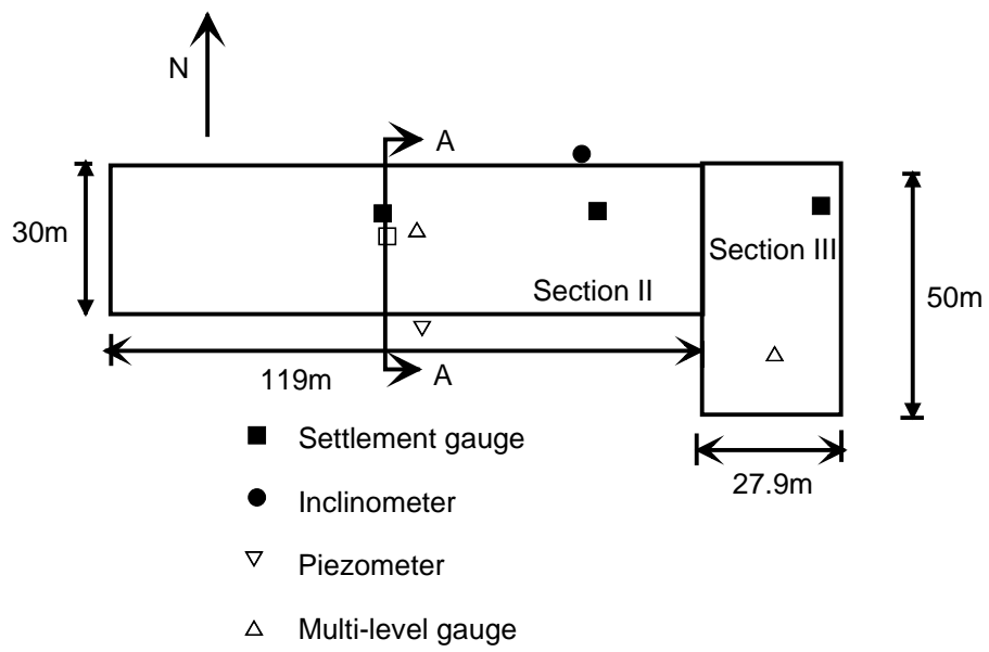
Fig. 6. Embankment plan view with field instrumentation(After Chu and Yan 2005)
