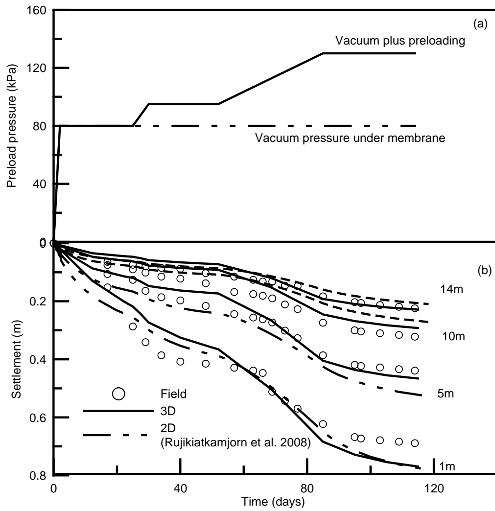
Fig.9. (a) Loading history and (b) Consolidation settlements
