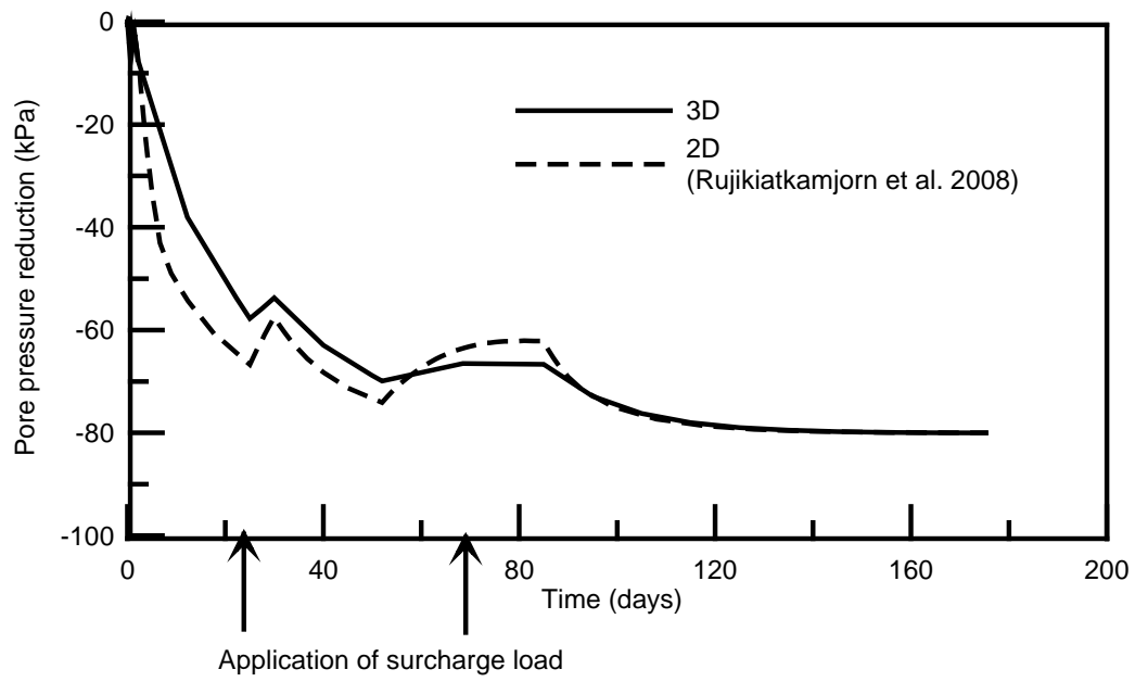
Fig. 10 Pore pressure variation (Section III) at 0.25m away from the embankment centerline at 5.5m depth (arrows indicate times when surcharge loads were applied)
