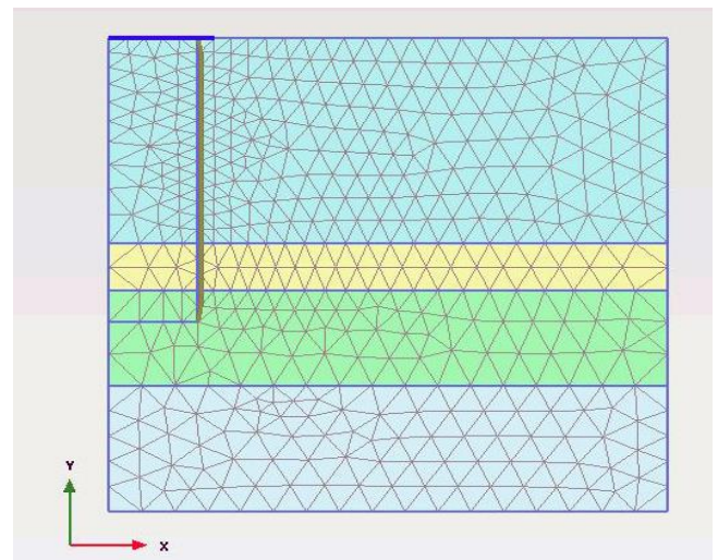
Figure 29 Typical Mesh PLAXIS 2D
