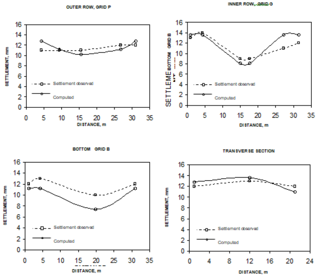
Figure 19 Observed Settlement Vs Computed Value at Various Section
