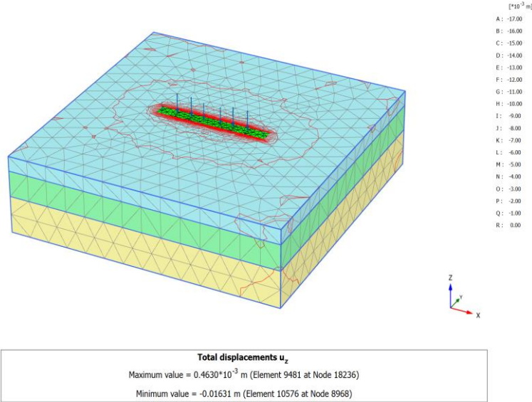
Figure 23 Settlement Contour
