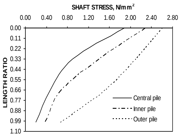
Figure 17(a) Variation of stress along the shaft of typical piles along the center line of raft for 8.10kN
