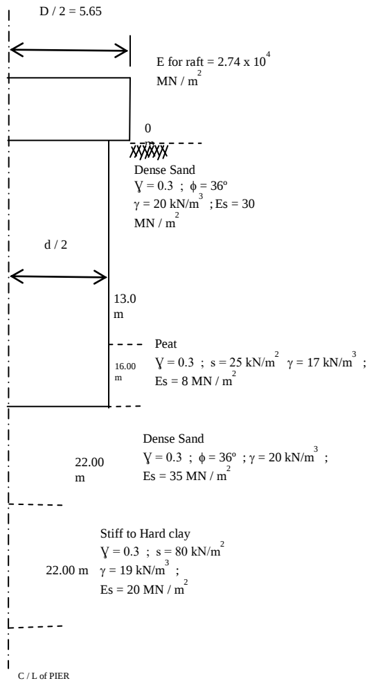
Figure 27(b) Pier &amp; Geotechnical Data Hypothetical Problem
