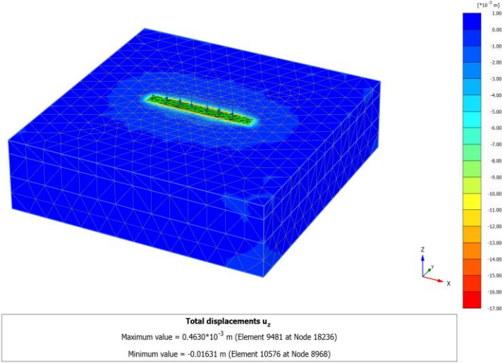
Figure 22 PLAXIS 3D Model
