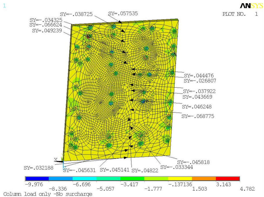
Figure 20 Raft contact stress along grid G
