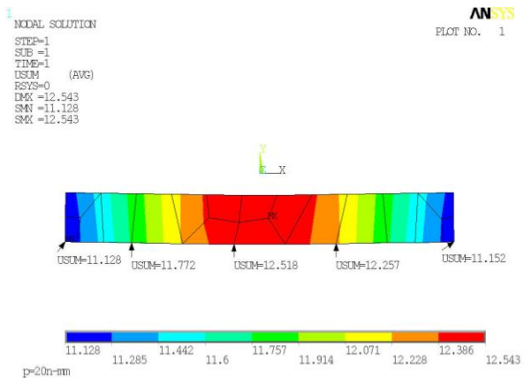
Figure 8(b) Settlement of piled raft at the load of 1.55 kN
