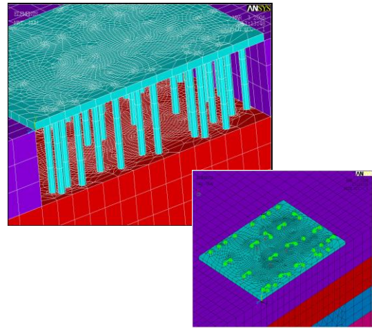
Figure 18 Finite Element Simulation and Meshing of Piled Raft
