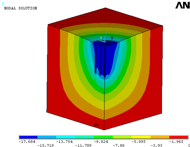
Figure 11 Settlement contour for a circular piled Raft for the load of 8.1 kN
