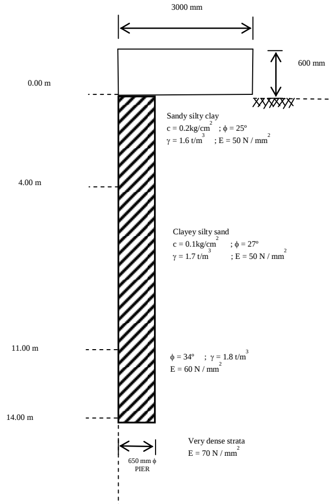
Figure 27(a) Observational study G 13 Pile group model
