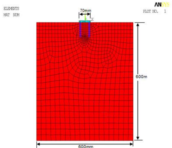
Figure 8(a) Rectangular piled raft model with finite element mesh used in plane strain analysis of ANSYS
