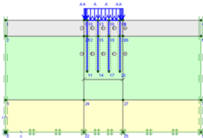
Figure 25 PLAXIS model for Pier
