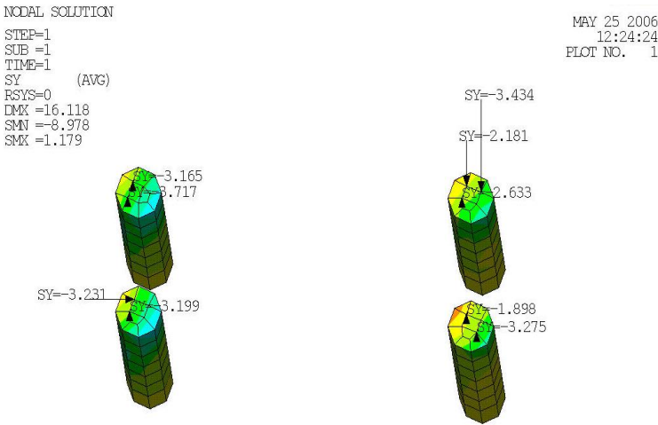
Figure 21 Typical head stress values
