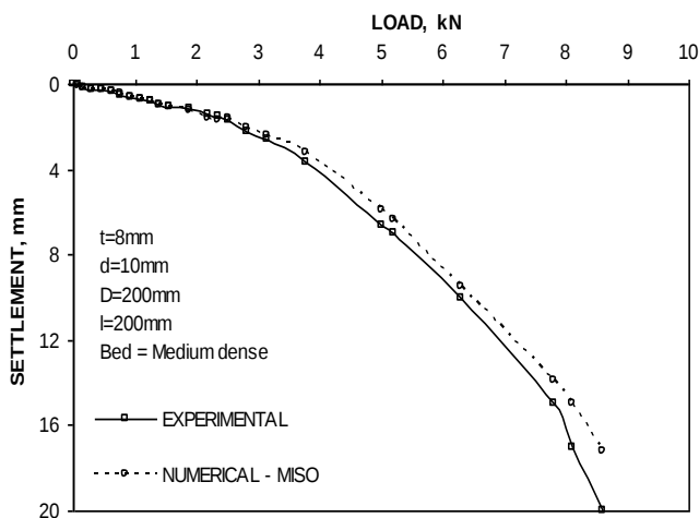
Figure 12 Comparison of load-settlement behaviour between ANSYS and model test data (Circular Raft)
