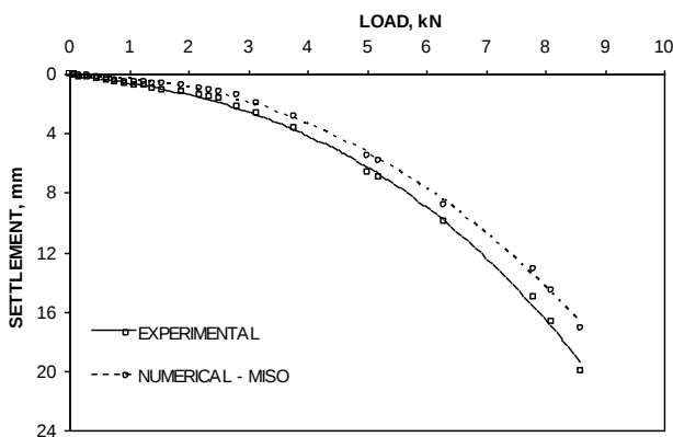
Figure 7 Comparison of load-settlement behaviour between numerical and 1g model test data ( D=200\text{mm} , t=8\text{mm} , d=10\text{mm} and l=100\text{mm} )
