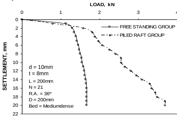
Figure 1 Comparison of load-settlement response of free standing pile group and pile group of piled raft
