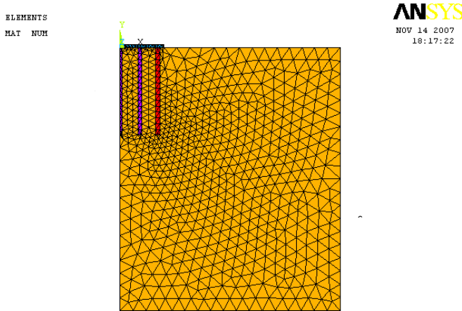
Figure 6 Axisymmetric model and mesh used in ANSYS analysis
