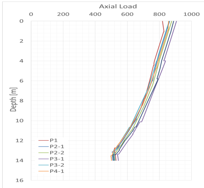
Figure 24 Pile Shaft Stress Distribution
