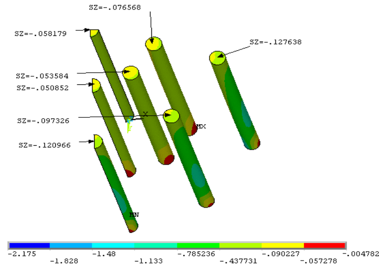
Figure 16 Stresses in pile tips for the load of 2.1 kN (Settlement =1.8mm)
