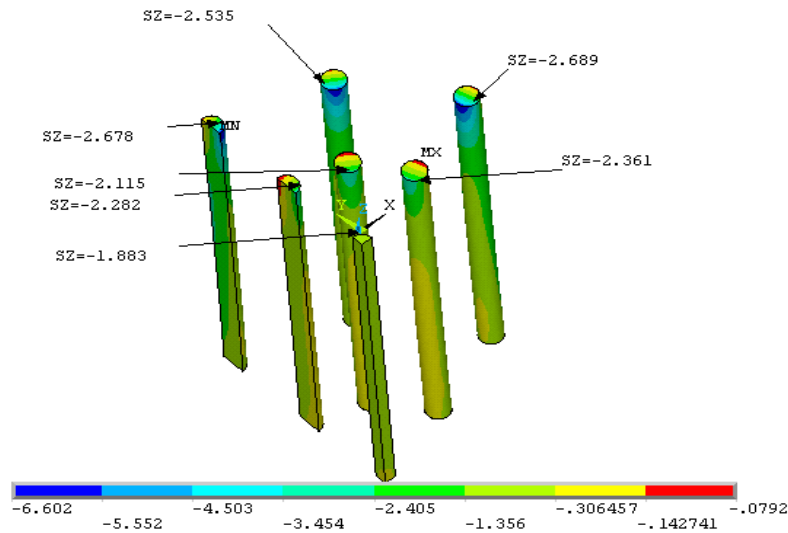
Figure 15 Pile Head stress for the load of 8.1 kN (settlement =17.8mm)
