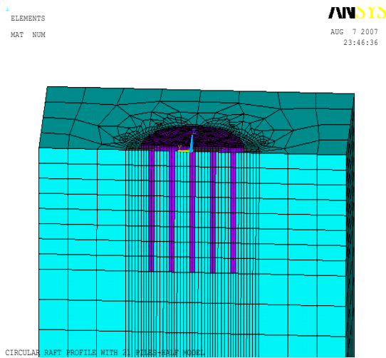
Figure 4 Finite element mesh for piled raft (linear analysis)
