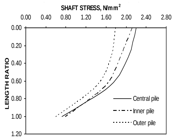
Figure 17(b) Variation of stress over the length of pile of square piled raft for the load of 8.7kN (No. of piles 25 at 4d spacing)
