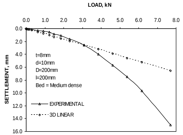
Figure 5 Comparison of load – settlement response between ANSYS (linear) and model test results for circular piled raft
