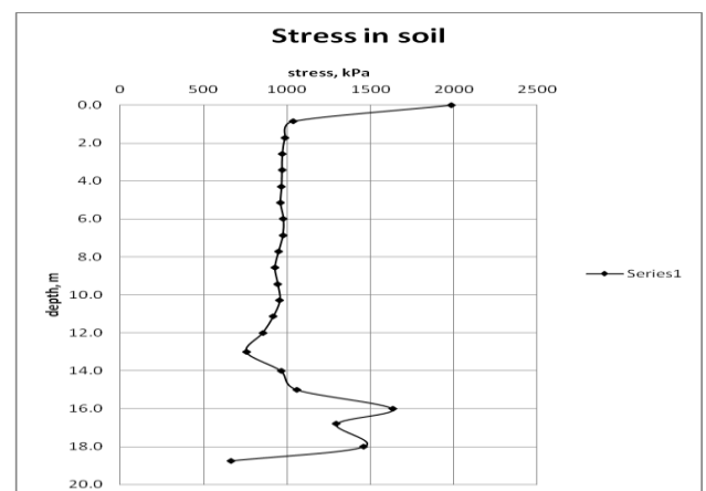
Figure 30 Shaft Stress Mobilisation (18m Deep Pile)
