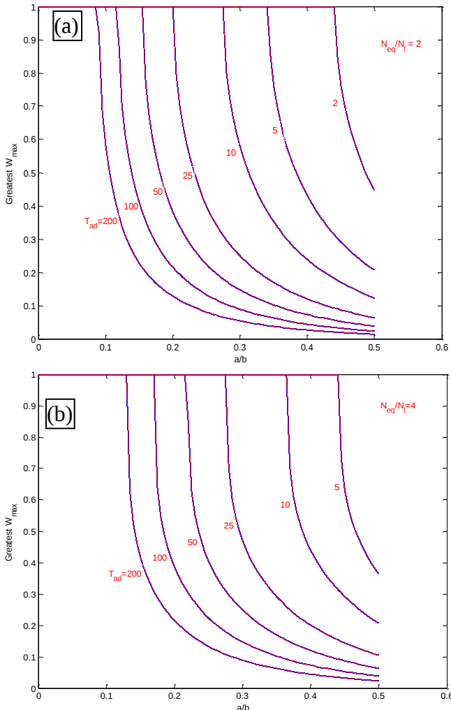
Figure 3 Relationship between greatest pore pressure ratio and drain system parameters for: (a) N_{eq}/N_l = 2 , (b) N_{eq}/N_l = 4 (redrawn after Seed and Booker, 1977)
