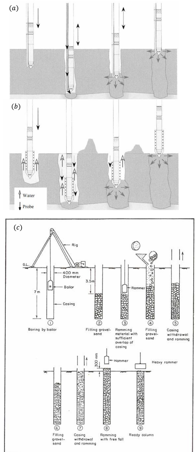
Figure 2 (a) Dry bottom-feed; (b) Wet top-feed method process (JGS, 1998), (c) Cased-borehole method (after Datye and Nagaraju, 1975)
