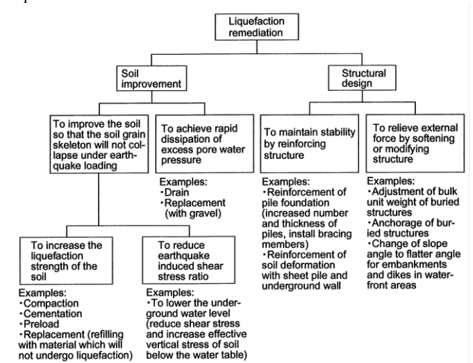
Figure 1 Strategy to be considered for liquefaction remediation (PIANC, 2001)
