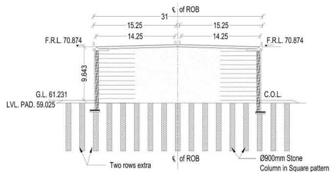
Figure 10 Typical ground improvement scheme adopted for ROB site in Bongaigaon
