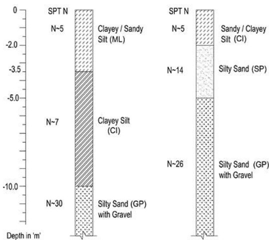
Figure 8 Typical soil profiles at the ROB sites in Bongaigaon
