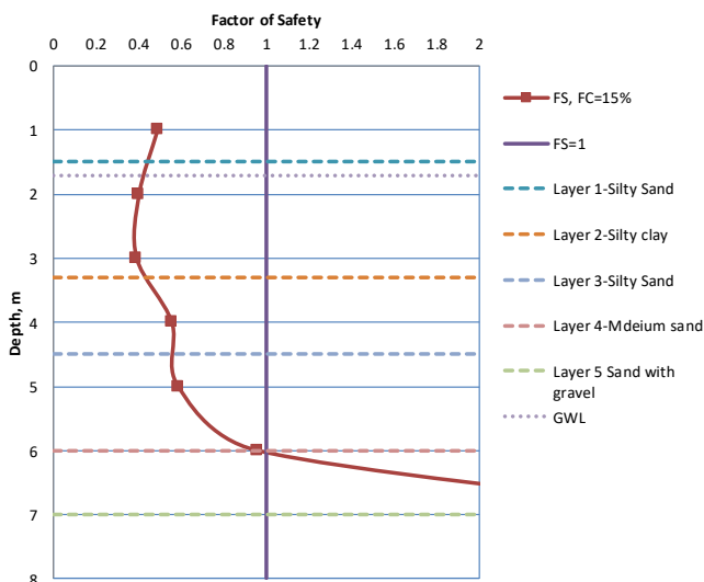
Figure 9 Typical liquefaction potential analysis (factor of safety variation) at ROB site
