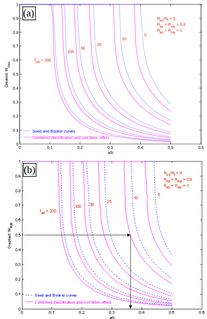
Figure 4 Design curves considering densification and soil fabric effect (a) N_{eq}/N_l of 3 (b) N_{eq}/N_l of 4, (after Krishna et al. 2014)
