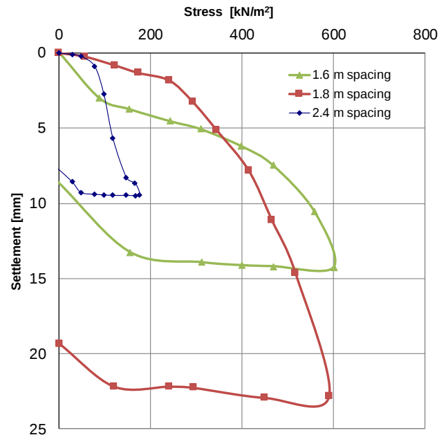
Figure 7 Load test results on stone column reinforced ground with different configurations
