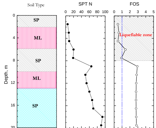
Figure 6 Typical soil profile and liquefaction potential evaluation
