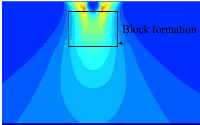
Figure 8: Vertical stress distribution under rough footing for spacing ratio S/B=1.25 corresponding to semi-infinite soil layer
