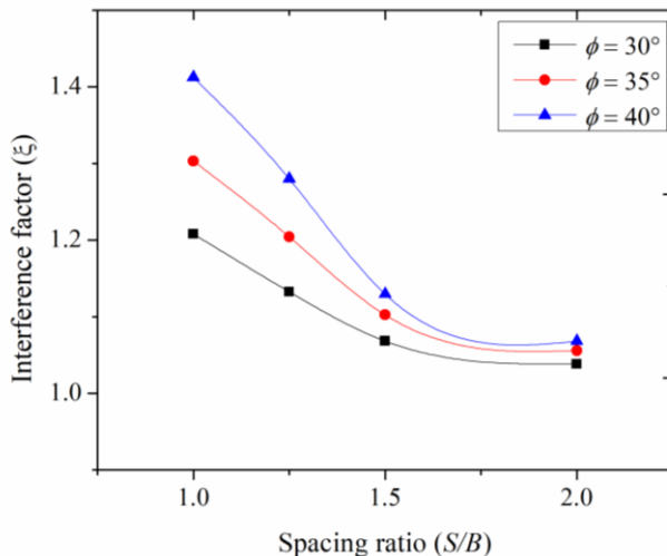
Figure 11: Variation of interference factor with spacing ratio for rough square footing corresponding to H/B = 0.5
