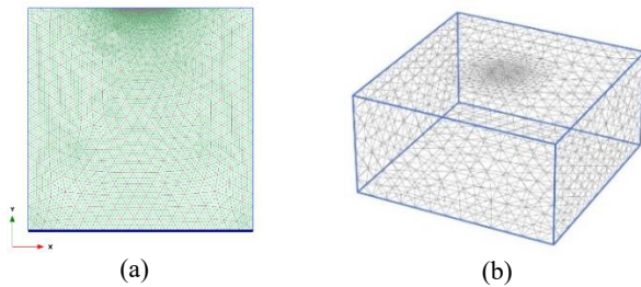
Figure 3: Mesh configuration used for (a) PLAXIS 2D model, and (b) PLAXIS 3D model
