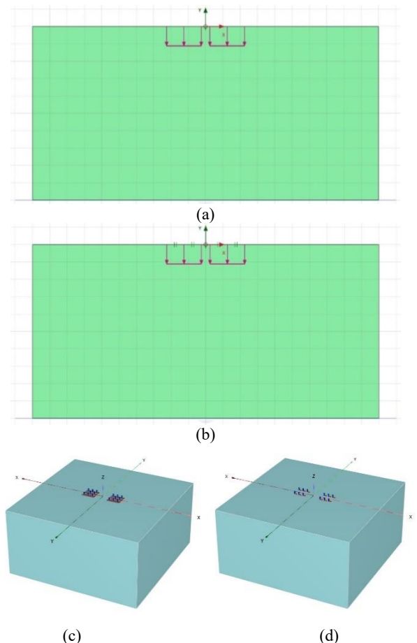
Figure 2: Models of closely-spaced footings: (a) PLAXIS 2D model for the case of smooth strip footings, (b) PLAXIS 2D model for the case of rough strip footing, (c) PLAXIS 3D model for the case of square footings, and (d) PLAXIS 3D model for the case of circular footings
