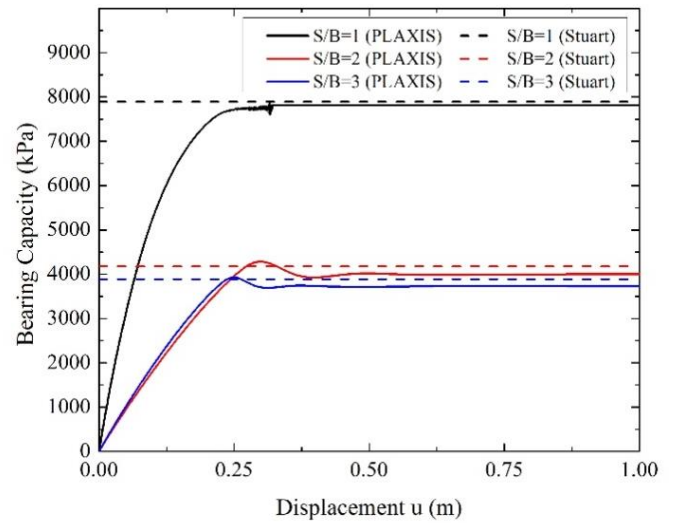
Figure 4: Comparison of bearing capacity of footing from present model with Stuart (1962)
