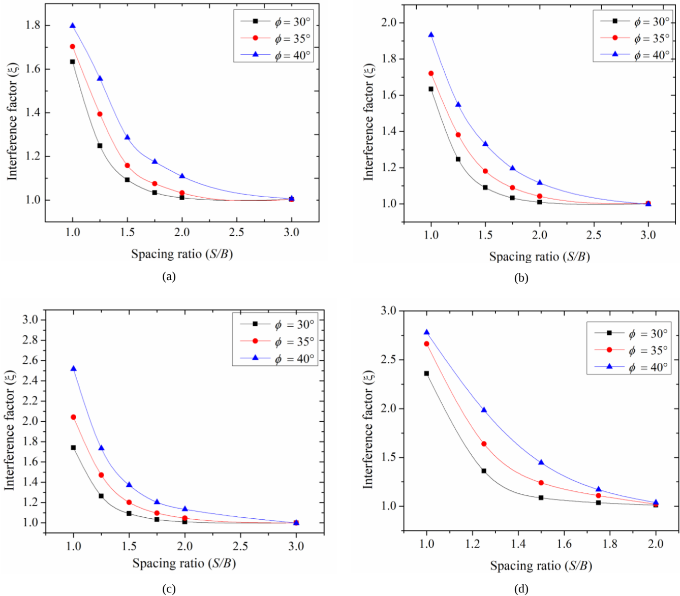
Figure 5: Variation of interference factor with S/B ratios for different angles of shearing resistance of sand in the case of smooth footing for (a) semi-infinite, (b) H/B=1 , (c) H/B=0.75 , and (d) H/B=0.5
