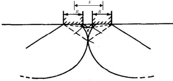
Figure 7: Failure surfaces of closely-spaced rough footings forming "block" (modified after Stuart 1962)
