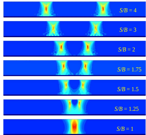
Figure 9: Vertical stress distribution under rough footing for various spacing ratios corresponding to H/B=1
