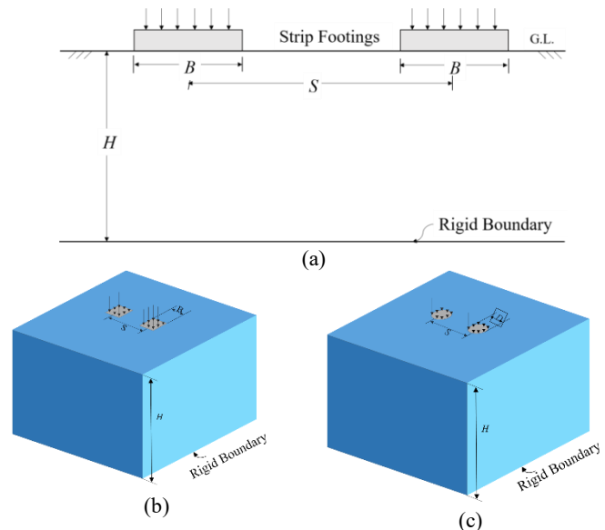
Figure 1: Schematic diagram of the closely-spaced (a) strip (b) square, and (c) circular footings
