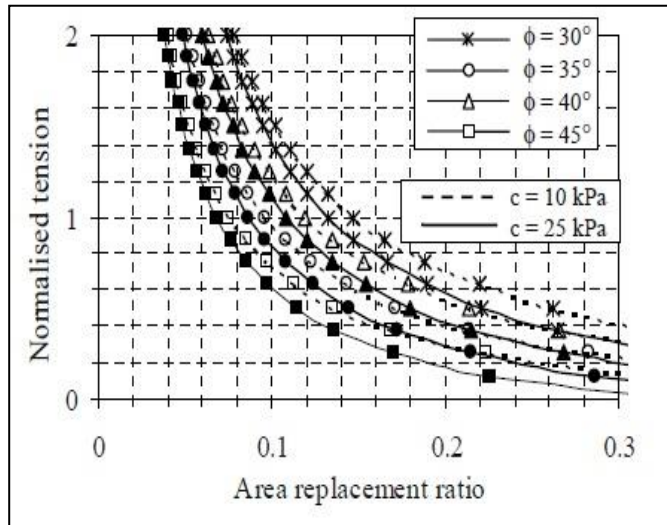
Figure 7 Design Chart for Geosynthetic Encased Stone Column after Murugesan and Rajagopal (2008)
