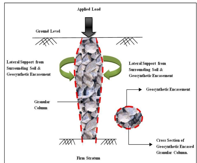
Figure 3 Single Encased Granular Column - Schematic Representation
