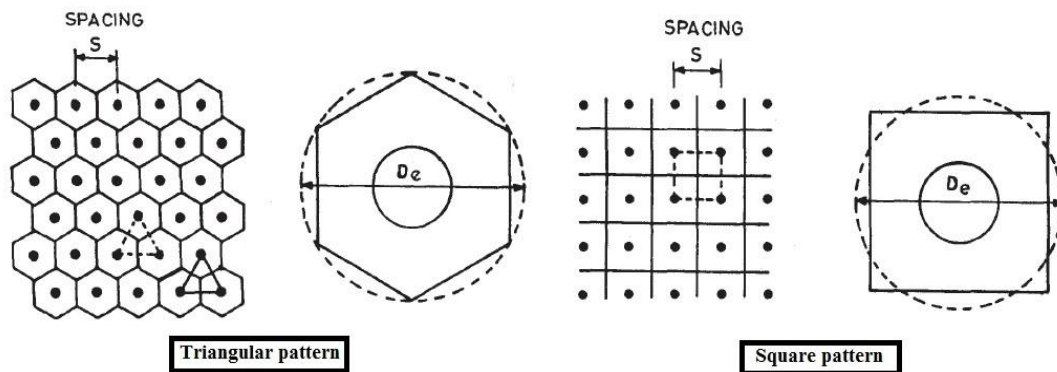
Figure 1 Various patterns of Stone Column Arrangement
