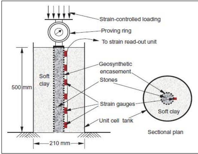
Figure 6 Unit cell load test on stone column after Murugesan and Rajagopal (2007)
