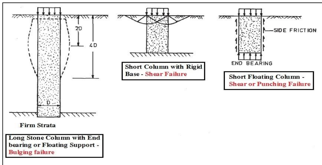
Figure 2 Failure Mechanisms of a Single Stone column
