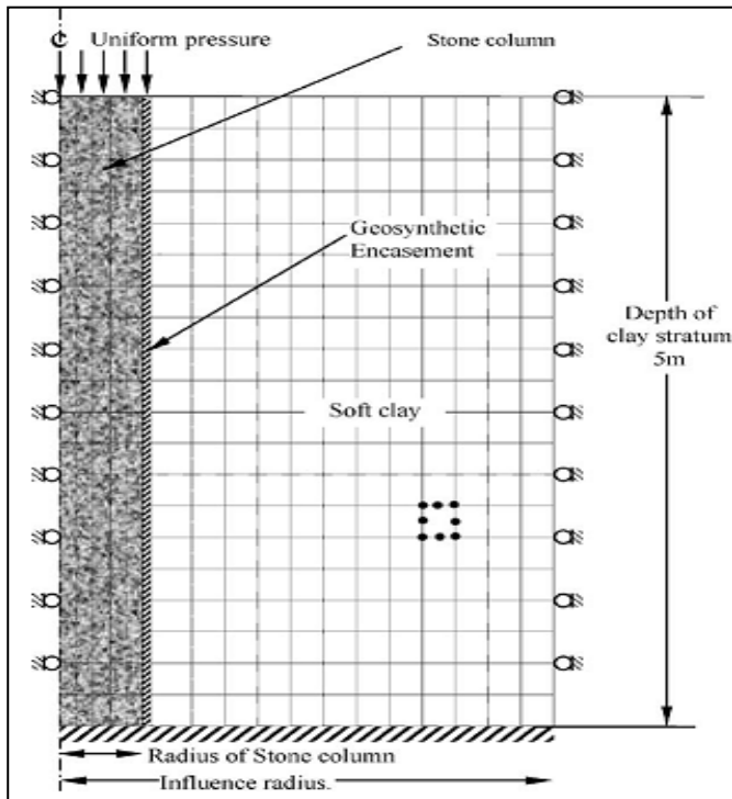
Figure 5 Typical Finite Element Mesh of Encased Stone Column after Murugesan and Rajagopal (2006)
