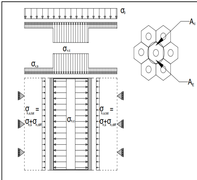
Figure 4 Analytical model of geotextile encased columns after Raithel & Kempfert 2000.
