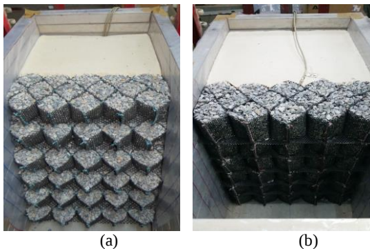
Figure 6 Photographs of the model retaining walls (a) battered wall (b) vertical wall
