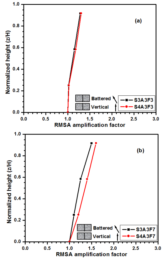
Figure 16 Variation of RMSA amplification factors with normalized height showing the effect of sloping angle in geocell configuration for battered and vertical walls for 0.3g (a) 3 Hz (b) 7 Hz
