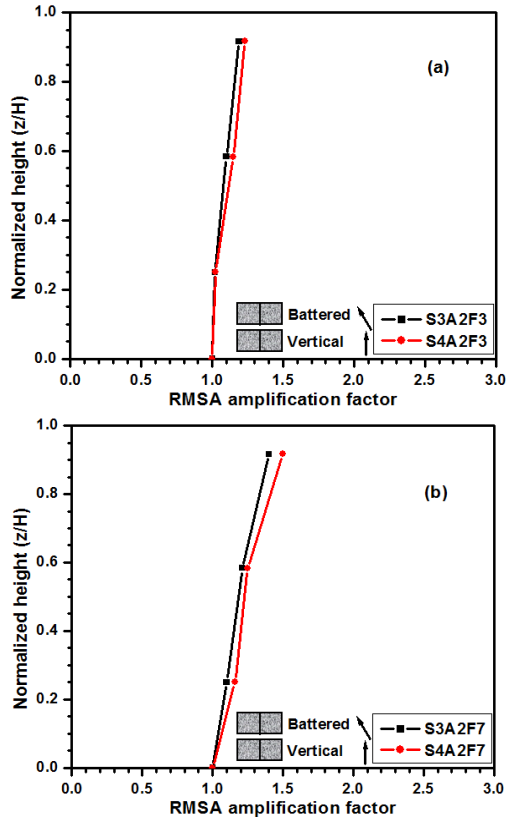
Figure 14 Variation of RMSA amplification factors with normalized height showing the effect of sloping angle in geocell configuration for battered and vertical walls for 0.2g (a) 3 Hz (b) 7 Hz
