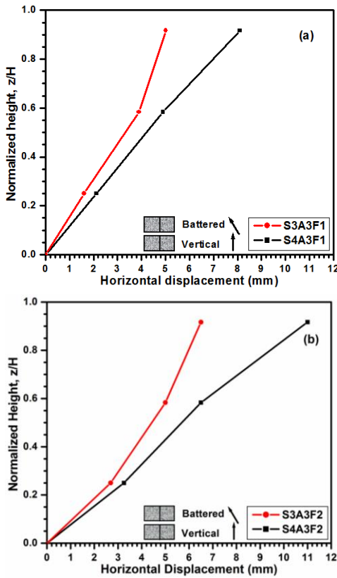
Figure 11 Variation of horizontal displacement of the wall facing for normalized height showing the effect of slope angle in geocell configuration for battered and vertical walls at 0.3g (a) 1Hz (b) 2 Hz
