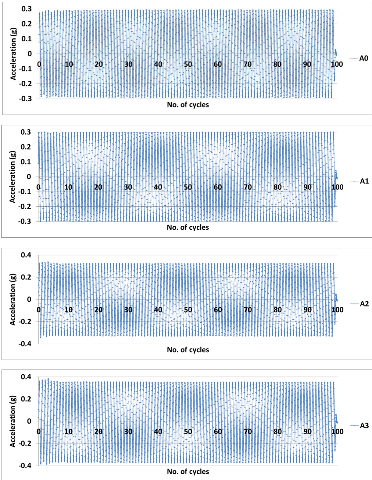
Figure 7 Typical acceleration response from a model test
