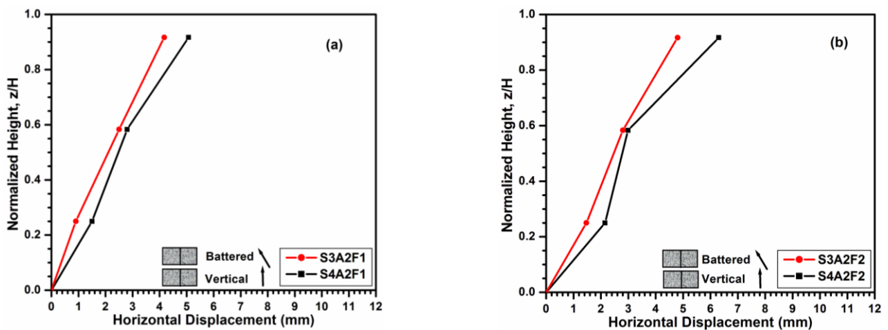
Figure 9 Variation of horizontal displacement of the wall facing for normalized height showing the effect of slope angle in geocell configuration for battered and vertical walls at 0.2g (a) 1Hz (b) 2 Hz
