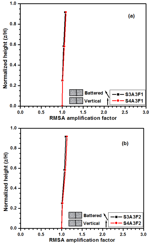
Figure 15 Variation of RMSA amplification factors with normalized height showing the effect of sloping angle in geocell configuration for battered and vertical walls for 0.3g (a) 1 Hz (b) 2 Hz
