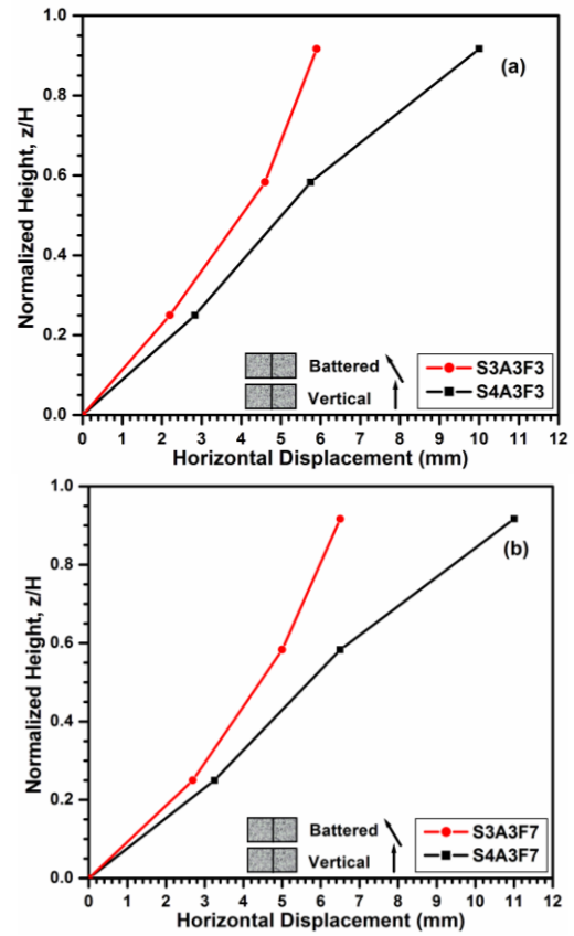
Figure 12 Variation of horizontal displacement of the wall facing for normalized height showing the effect of slope angle in geocell configuration for Set3 and Set4 for 0.3g (a) 3Hz (b) 7 Hz
