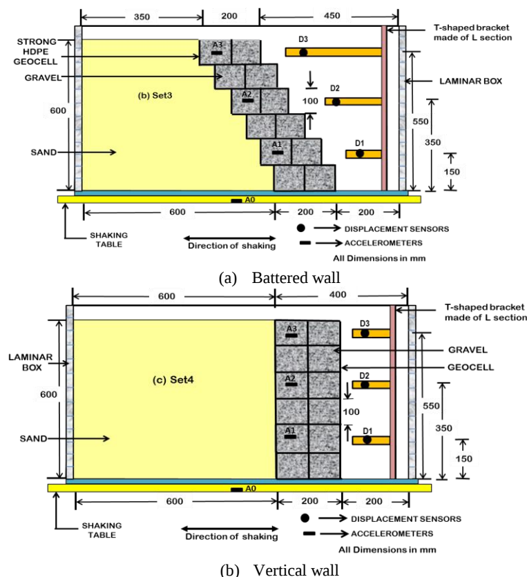
(b) Vertical wall (c) Figure 5 Schematic diagrams of the model retaining walls
