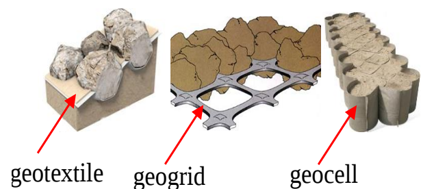
Figure 1 Mechanisms of interaction of different types of geosynthetics with soil/aggregate (compiled from google images)
