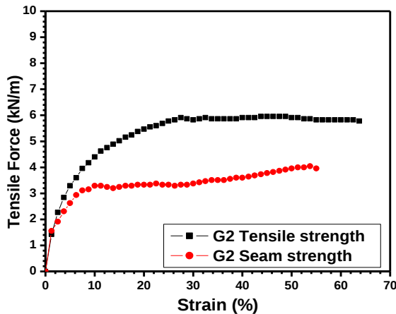
Figure 4 Load-elongation response of geonet
