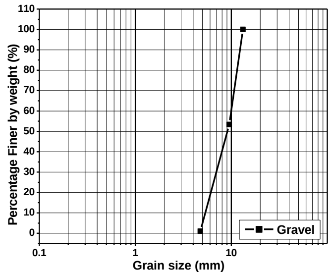
Figure 3 Grain size distribution of gravel
