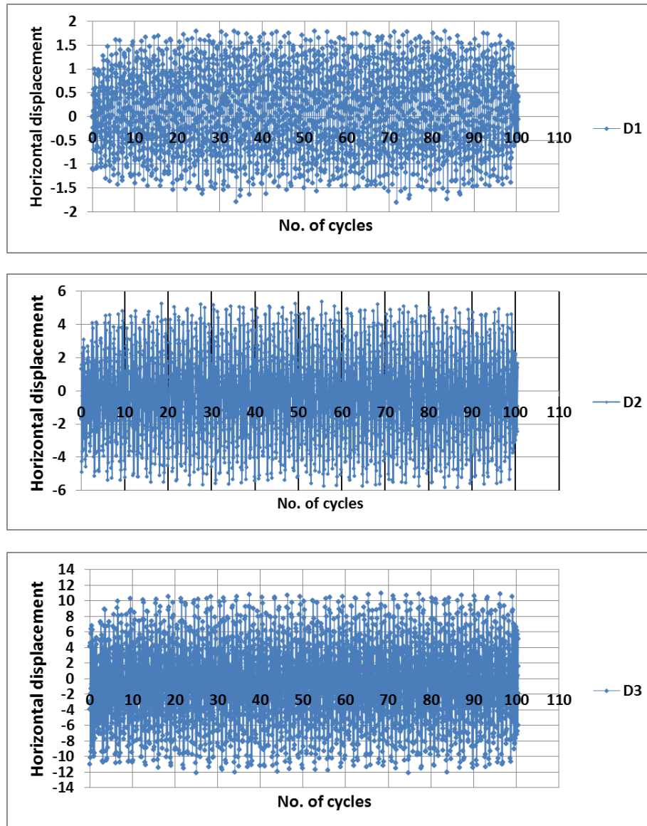
Figure 8 Typical displacement response from a model test
