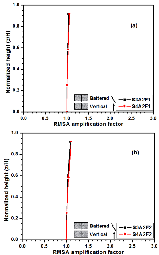
Figure 13 Variation of RMSA amplification factors with normalized height showing the effect of sloping angle in geocell configuration for battered and vertical walls for 0.2g (a) 1 Hz (b) 2 Hz
