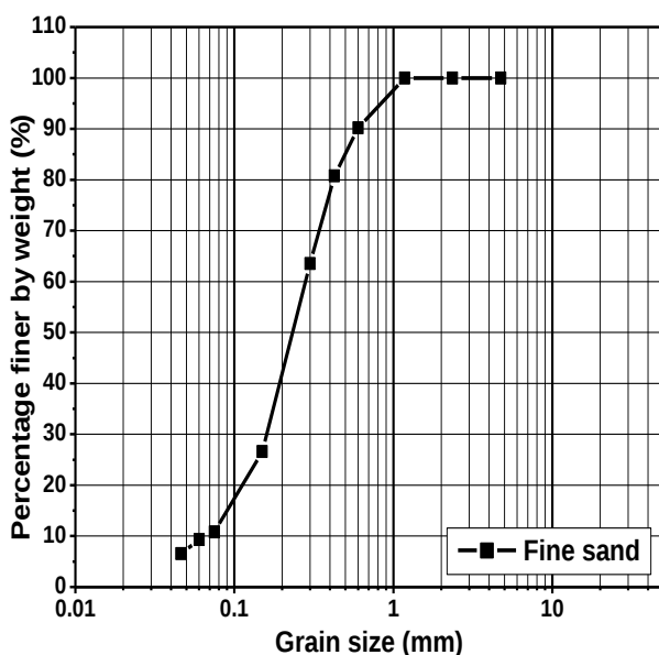
Figure 2 Grain size distribution of fine sand
