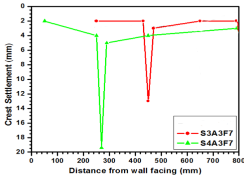
Figure 17 Variation of crest settlement with distance from the wall facing for battered and vertical walls at shaking of 0.3g and 7 Hz
