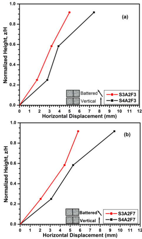
Figure 10 Variation of horizontal displacement of the wall facing for normalized height showing the effect of slope angle in geocell configuration for battered and vertical walls at 0.2g (a) 3Hz (b) 7 Hz
