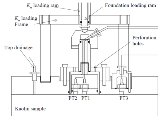
(b) Footing arrangement
