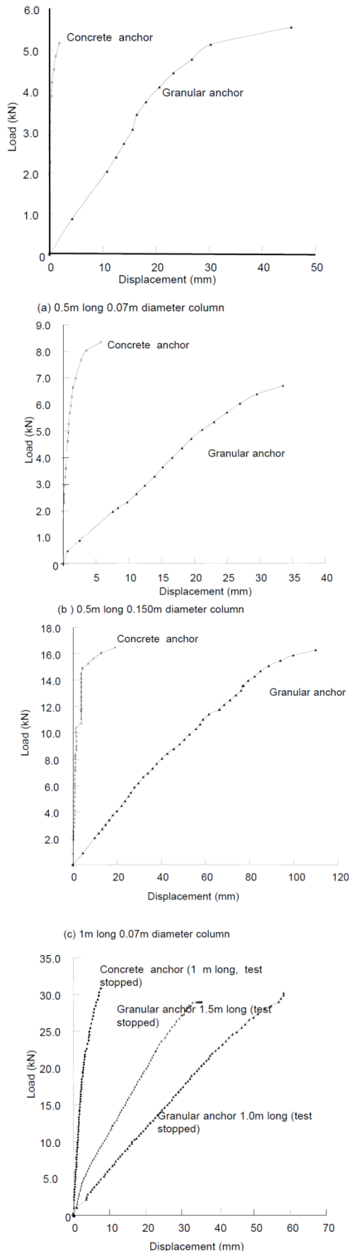
Figure 24 Load-displacement characteristics of concrete and granular anchors
