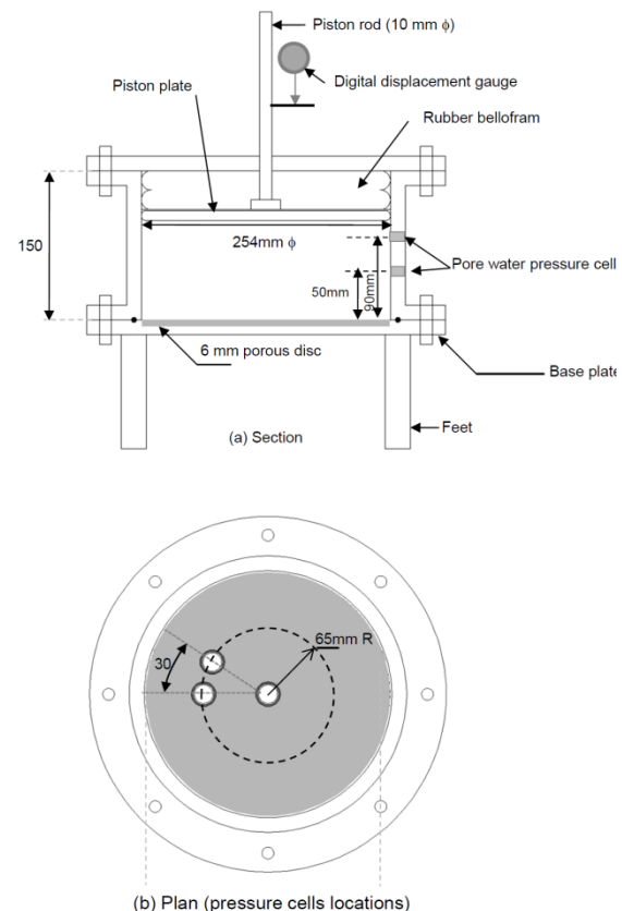
Figure 18 Schematic of one dimensional testing chamber
