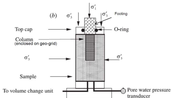
Figure 3 Testing arrangement where model footing is supported on granular column contained in geo-grid
