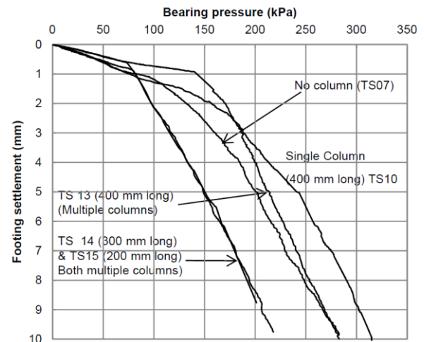
Figure 14 Bearing pressure–settlement relationships for an unreinforced clay bed and clay beds reinforced by a single end bearing column and column groups (floating and end bearing)
