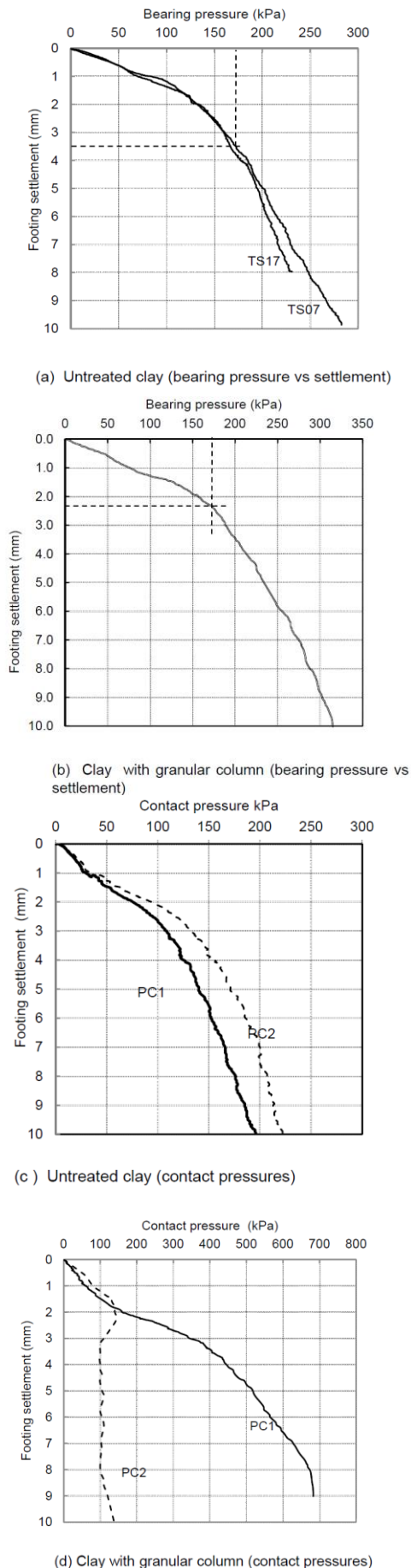
Figure 13 Bearing pressure vs settlement (Fully penetrating columns)
