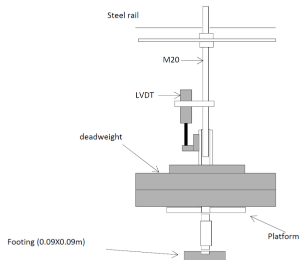
Figure 21 Foundation loading
