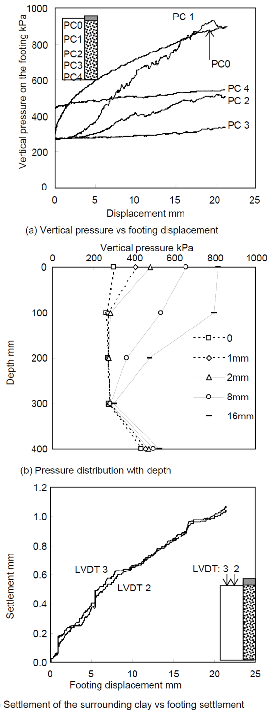
Figure 17 Performance of the sample with 50mm \square column during foundation loading
