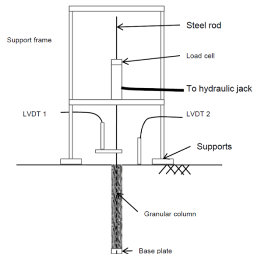
Figure 23 Schematic of loading frame
