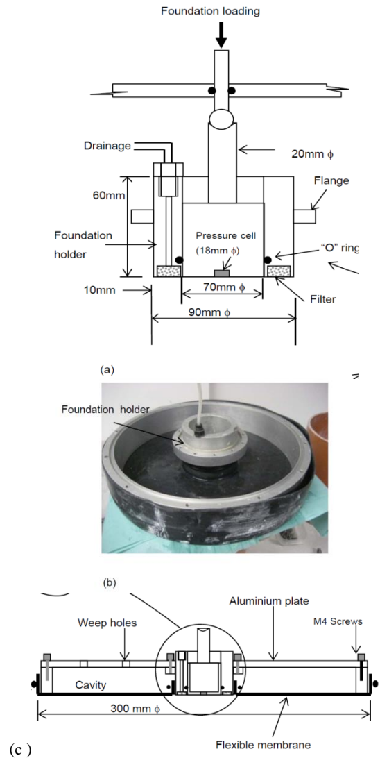
Figure 12 Footing and testing conditions away from footing
