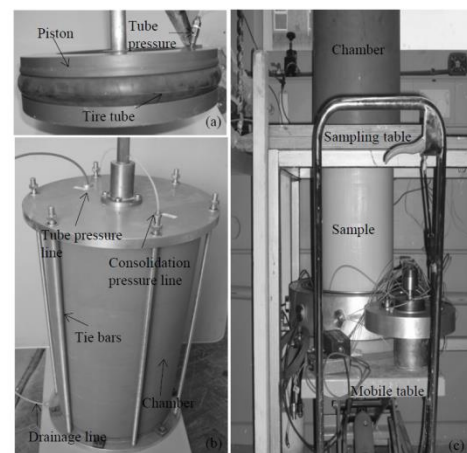
Figure 8 Sample preparation in one-dimensional consolidation chamber
