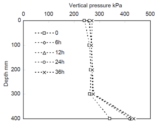
(b) Pressure distribution with depth
