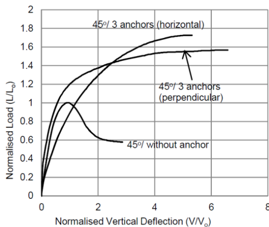
(a) Effects of horizontal and perpendicular columns
