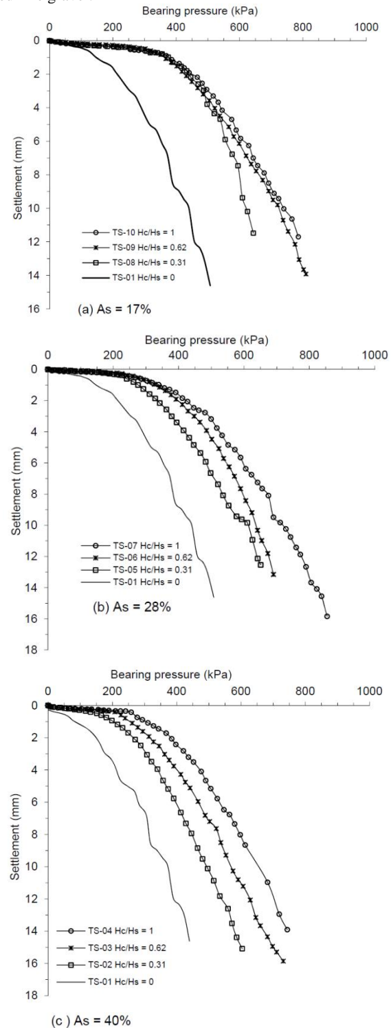
Figure 9 Displacement-bearing pressure for three area displacement ratio
