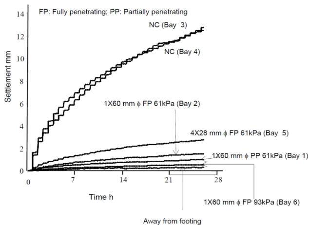
Figure 22 Settlement against time for loose sand bed
