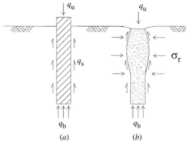
Figure 1 Solid and granular pile
