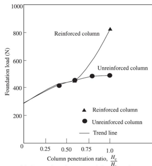
(b) Comparison between reinforced and unreinforced columns
