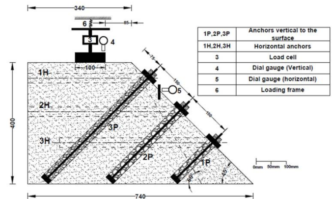
Figure 26 Cross-sectional view of the slope included with granular column anchors
