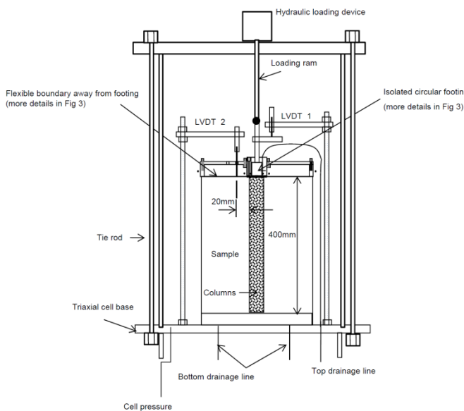
Figure 11 Testing chamber for assessing settlement of footing supported on circular footing under realistic boundary conditions
