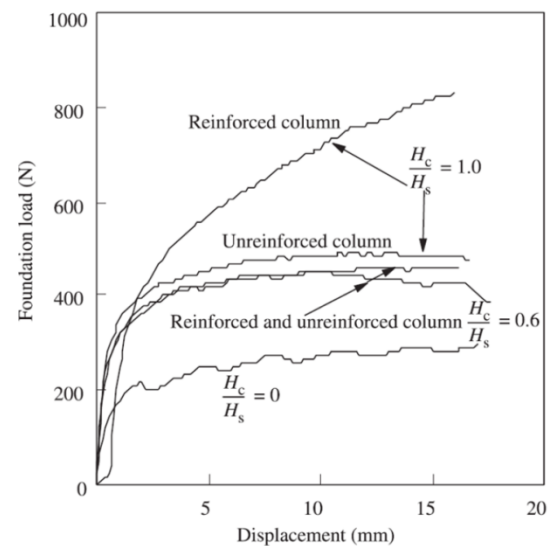
(a) Load vs displacement
