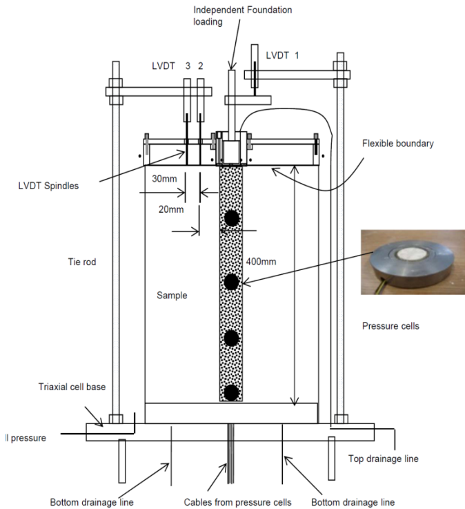
Figure 15 Assembled sample
