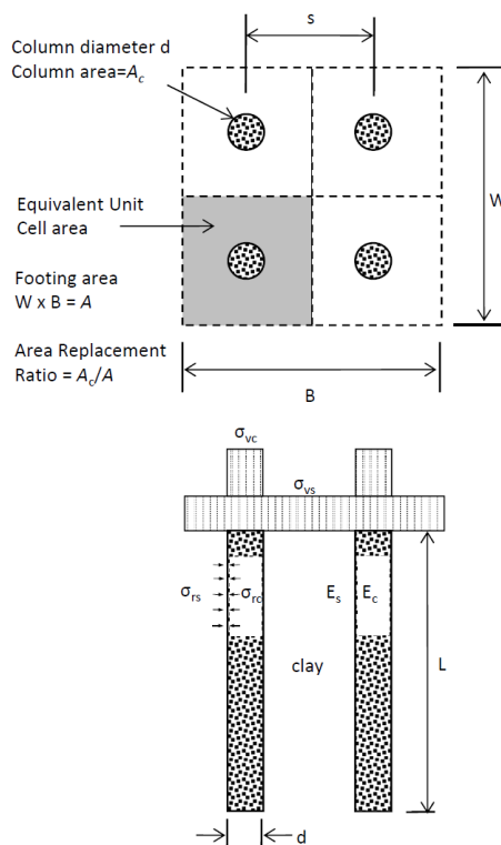
Figure 2 Key factors affecting granular column performance
