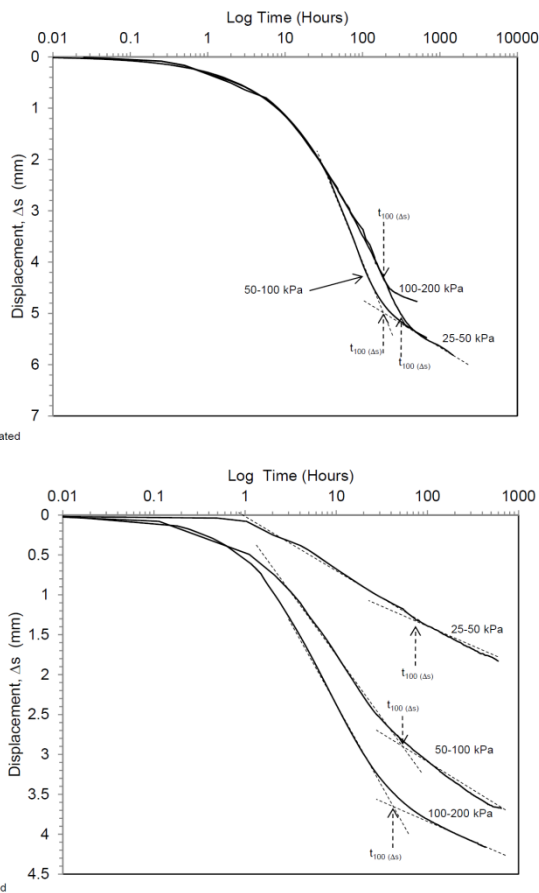
Figure 19 Settlement versus logarithm of time for silt with and without granular column
