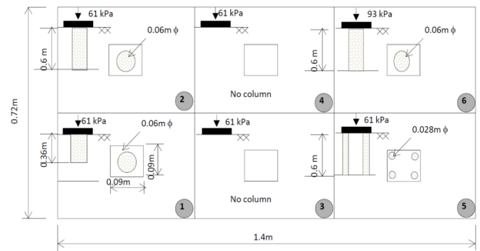
Figure 20 Footing Layouts
