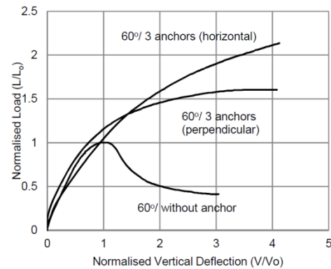
(c) Steep slope
