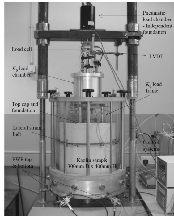
(a) Testing chamber
