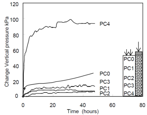
(a) Vertical pressure kPa
