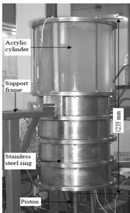
(a) Consolidation chamber
