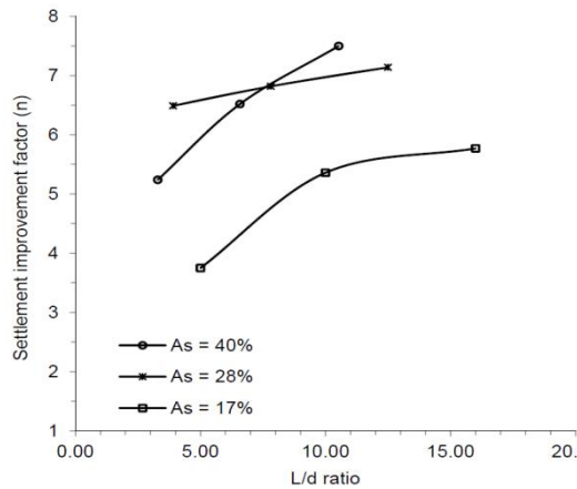
(a) Settlement improvement factor n vs A_s
