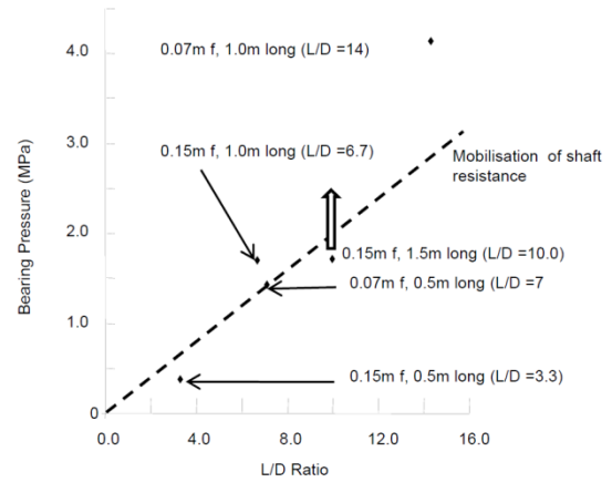
Figure 25 Bearing pressure vs L/D ratio QUB site
