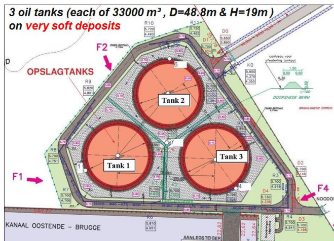
Figure 1 Overview of the site and location of the three tanks at Ostend (Belgium).
