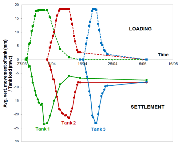
Figure 22 Average settlement of the tank during the hydro test.
