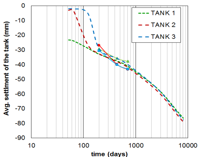
Figure 33 Predicted (lines) versus measured (dots) average settlement of the tanks under operational load.
