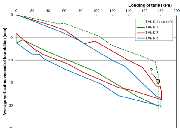
Figure 23 The full load-settlement curves for each of the oil tanks at hydro testing with unloading.
