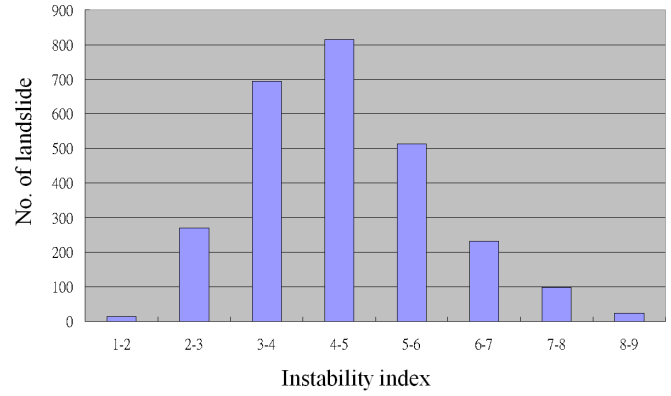
Figure 9 Distribution of the rated instability indices of the 2658 landslides
