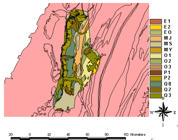
Figure 2 Distribution of screened ground variation data from SWCB (2000)
