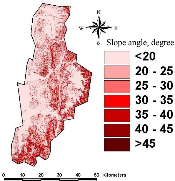
Figure 8 Distribution of slope angle factor with distinctive range and treated as a categorical parameter
