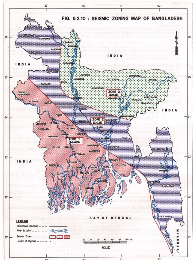
Figure 1 Seismic Zoning Map in BNBC-1993
