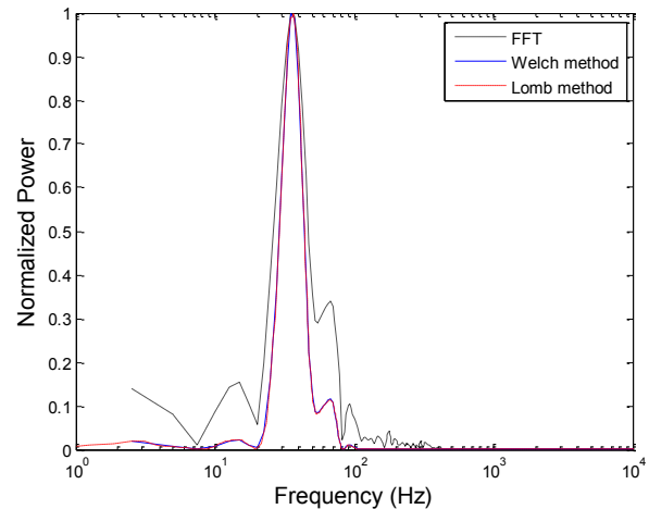
Figure 9. Normalized auto-spectral density estimated using various techniques (FFT, Welch method, Lomb method) for the filtered signal recorded at 45.1 meter depth at Richmond, BC (note: Lomb method corresponds to LSSA technique).
