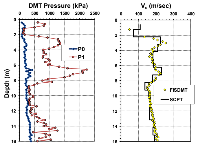
Figure 4. Frequent-interval SDMT soundings ( p_0 , p_1 , 0.2-m interval V_s ) and SCPT soundings (1-interval V_s ) at Treporti site.
