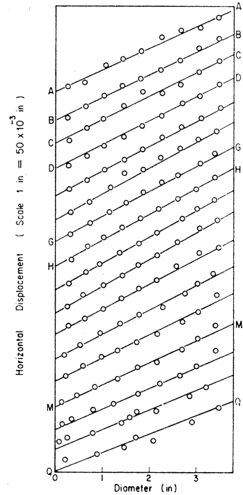
Fig. 19. Incremental horizontal displacement of markers plotted against their distances along the diameter for seventeen horizontal rows in plane 2 during isotropic consolidation.
