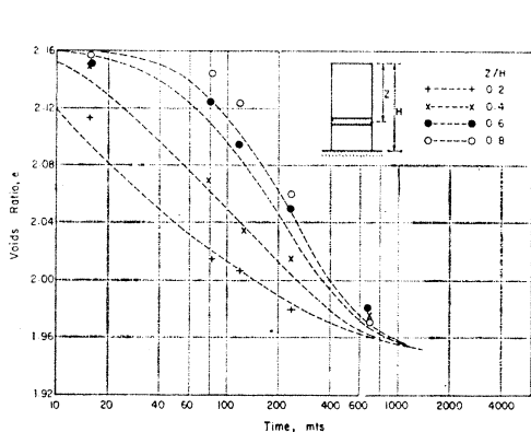
Fig. 11. Comparison of local voids ratios and the theoretical voids ratios at different depths during pore pressure dissipation for stress increment of 6 to 12 psi.
