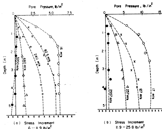
Fig. 13. Pore pressure isochrones determined from the local (a-b) measurements of voids ratios for two stress increments.
