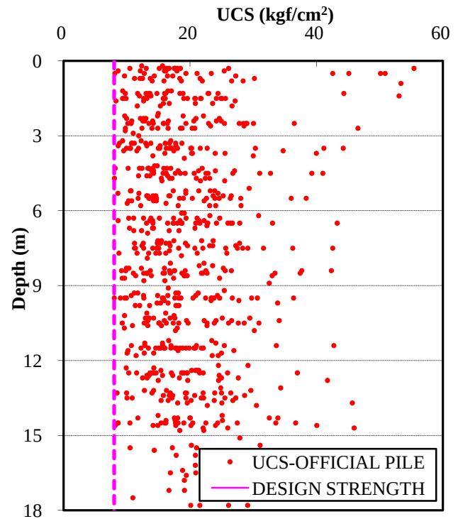
Figure 5 Profile of interpreted compressive strengths with depths of official piles
