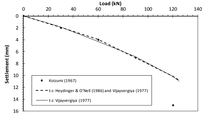
Figure 4 Comparison between the predicted and measured load - settlements for pile group
