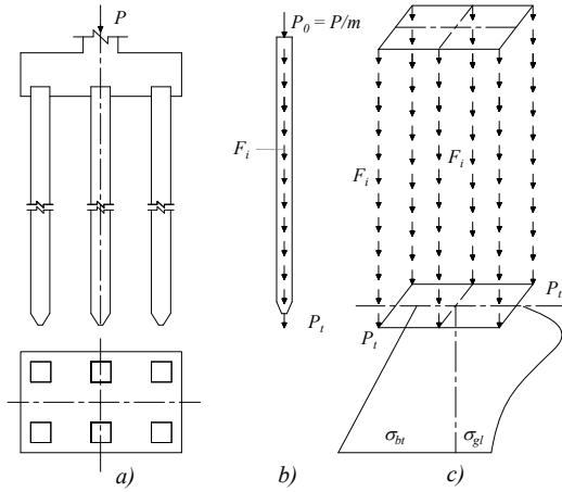
Figure 1 SDF Model with force on piles head are the same
