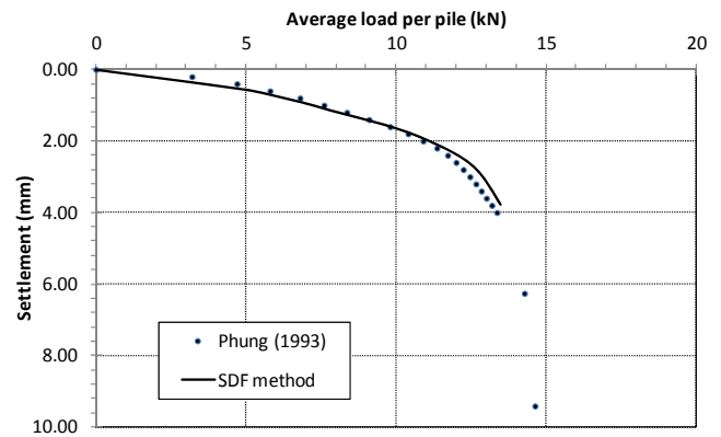
Figure 6 Comparison of the predicted and measured load – settlement behaviour for the pile group T2G
