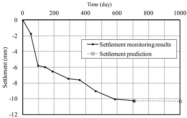
Figure 13 Settlement monitoring results of Amonia Storage Tank foundation
