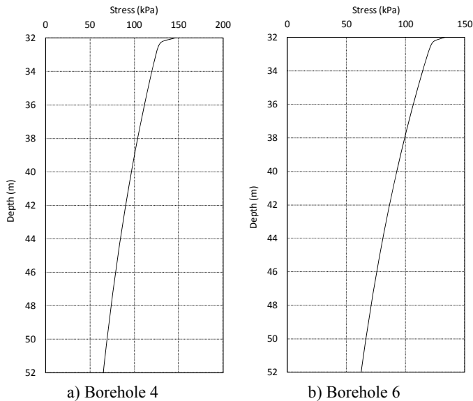
Figure 27 Soil Stress under pile tip plan
