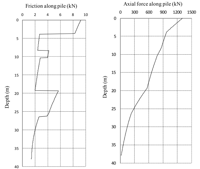
Figure 15 Pile skin friction and axial force
