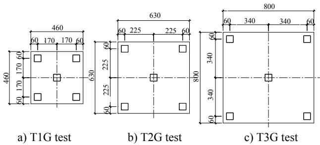
Figure 5 Model footings in plan
