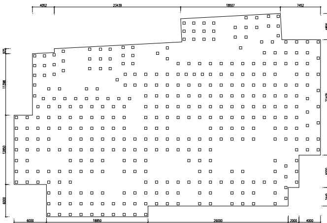
Figure 24 Pile Plan of Tower 2
