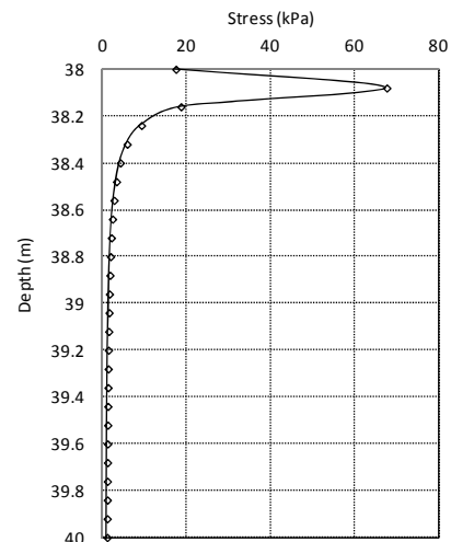
Figure 16 Maximum stress of soil under pile tip plan
