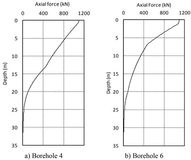
Figure 26 Axial force in pile
