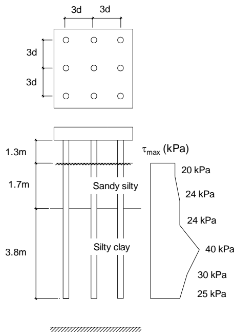
Figure 3 Full scale test presented by Koizumi et al (1967): layout of the pile group and subsoil model
