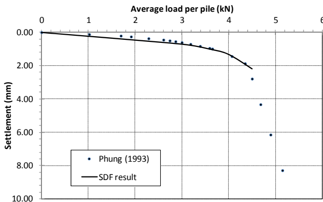
Figure 6A Comparison of the predicted and measured load – settlement behaviour for the pile group T1G
