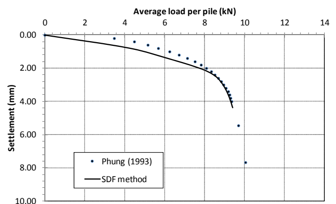
Figure 7 Comparison of the predicted and measured load – settlement behaviour for the pile group T3G
