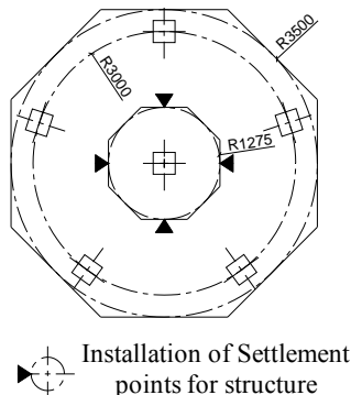
Figure 14 Pile plan and monitoring systems of Distillation Tower foundation
