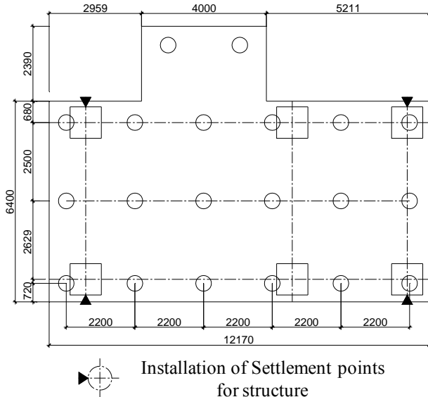
Figure 18 Pile plan and monitoring systems of Amonia Unit – Amonia Compressor
