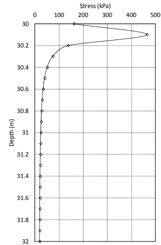
Figure 20 Maximum stress of soil under pile tip plan
