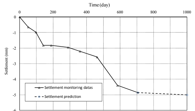
Figure 17 Settlement monitoring results of Distillation Tower foundation
