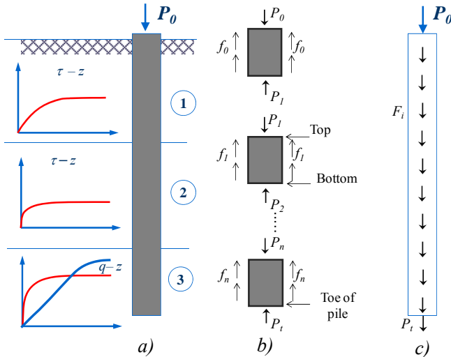
Figure 2 Distribute force in the pile
