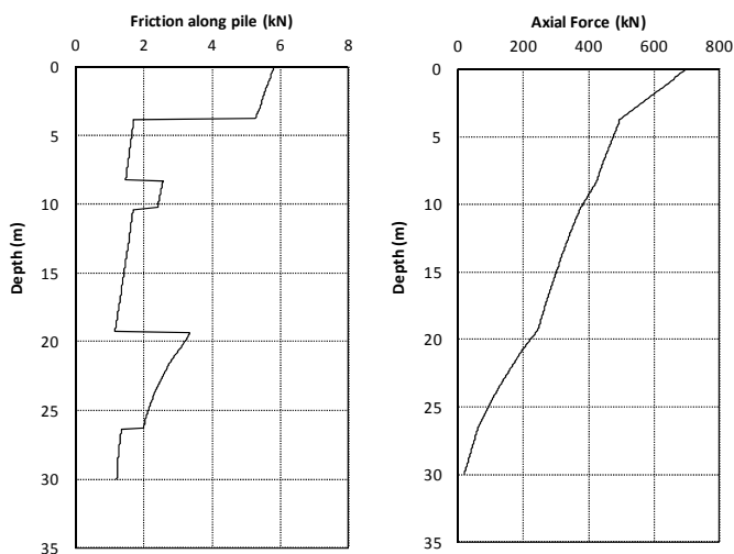
Figure 19 Pile skin friction and axial force versus depth
