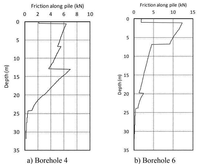
Figure 25 Friction along pile
