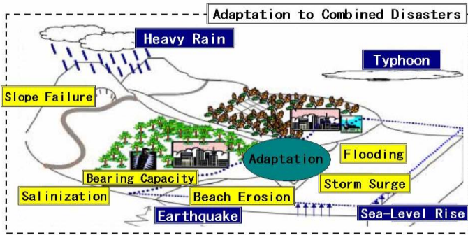
Figure 1 Examples of compound natural disasters (Yasuhara et al., 2012:2013)
