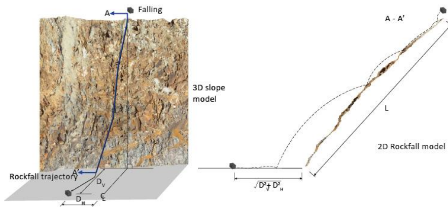
Fig. 7.38 Description of lateral dispersion ( D_H ) and extraction of 2D simulation section from 3D slope surface model
