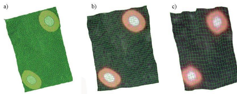
Fig. 4.8 3D surface models and 3D wireframe, D = 2.0 m (a), 5.0 m (b), 10.0 m (c) (Beaudesert Nerang road 1)
