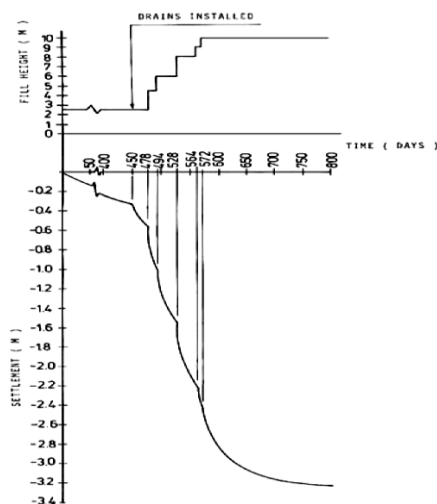
Fig. 6 Time-settlement curve at the coal storage yard, Port Kelang Power Station (Risseuw et al. , 1986)
