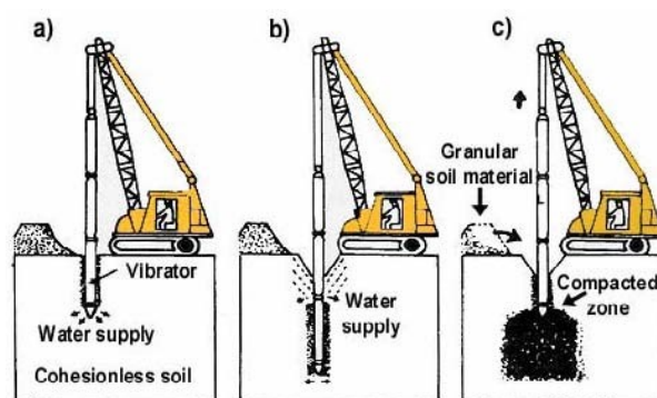
Fig. 20 Vibro compaction process
