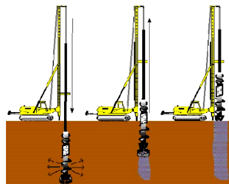
Fig. 30 Installation of CMC by displacement
