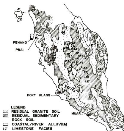
Fig. 3 Geological map of Peninsular Malaysia (Ting, 1985)
