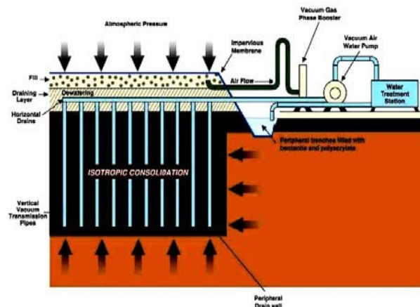
Fig. 9 Schematic layout of a vacuum consolidation system
