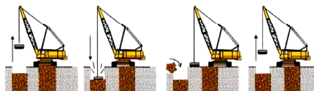
Fig. 27 Columns formed by dynamic replacement (DR) process
