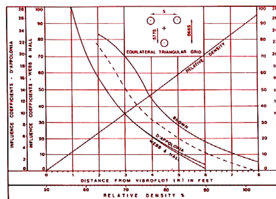
Fig. 21 Area pattern design chart (Glover, 1982)
