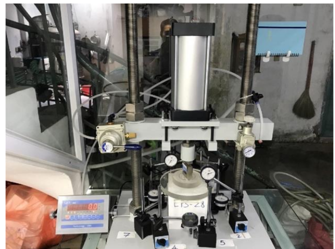
Investigation of Key Properties of EPS Geofoams for Highway Embankments on Soft Ground, after Tran-Nguyen and Phuoc (2022)
