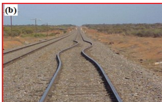
Figure 1(a) Ballast breakage in a rail track (b) Buckling of track due to insufficient lateral confinement (After Indraratna et al. 2011); (Quoted by Syed Khaja Karimullah Hussaini, Buddhima Indraratna, and J. S. Vinod, 2018)
