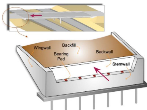
Figure 1. Typical seat type bridge abutment (After M. Ramalakshmi and G. R. Dodagoudar, 2018)
