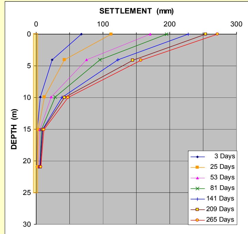
Vertical distribution of the settlement
