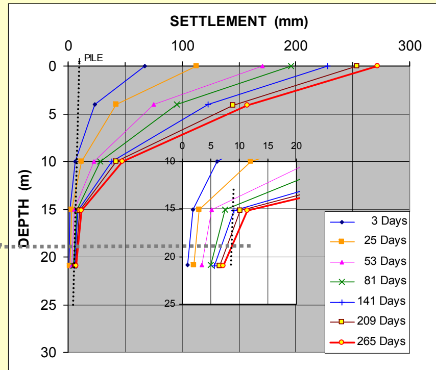
Settlement distribution
