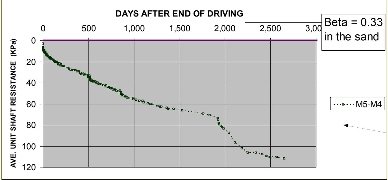
Average unit shaft shear in Piles PI and PII between Load Cells
