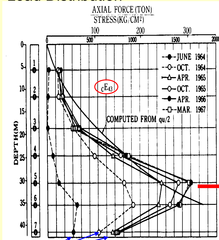
Load Distribution
