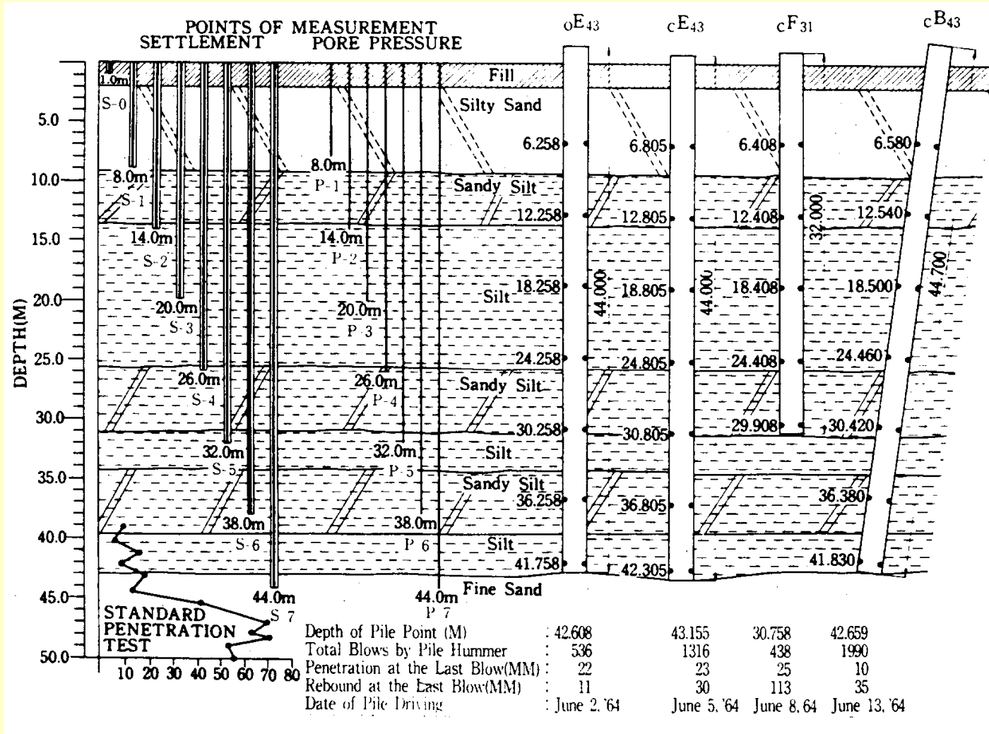
Profile of test site and piles
