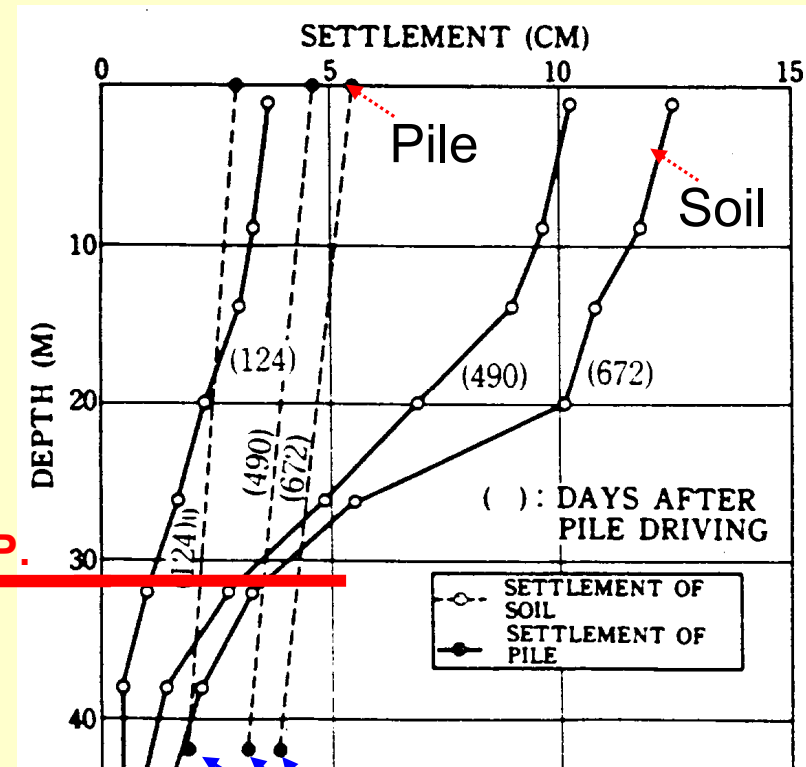
Settlement Distribution
