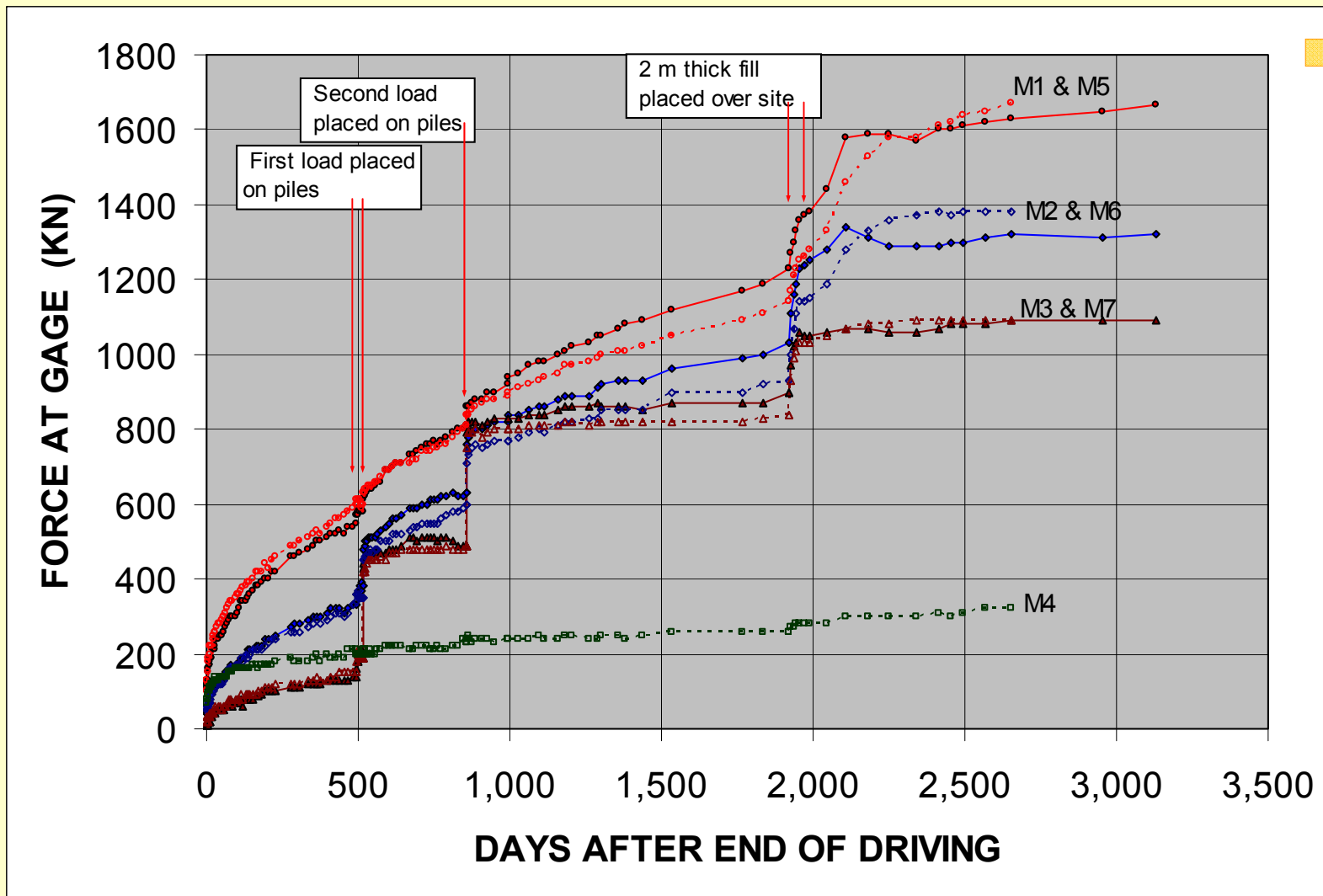
Measured loads in piles versus time after driving
