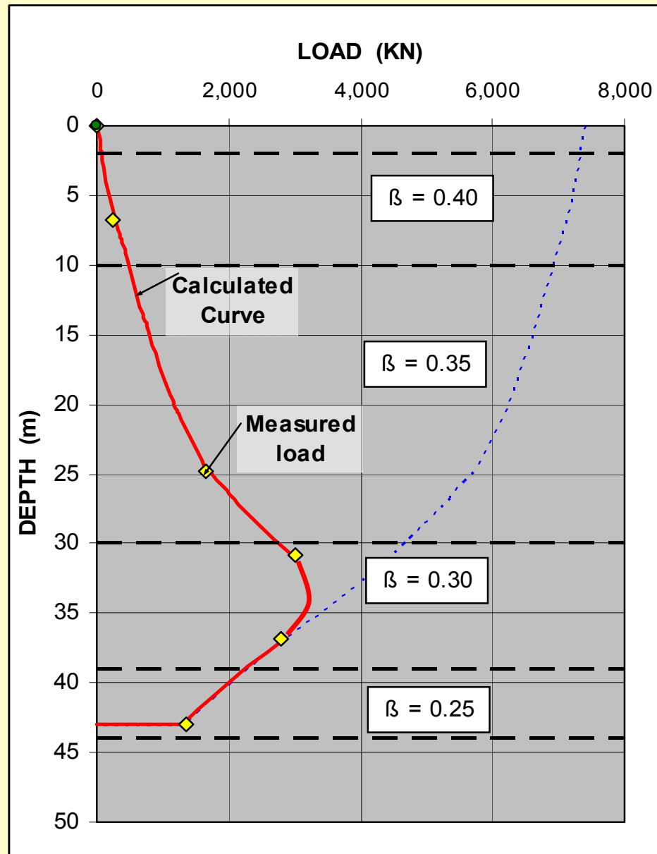
Measured load distribution and distribution matched to measured values in effective stress analysis. (Data from Endo et al., 1969).
