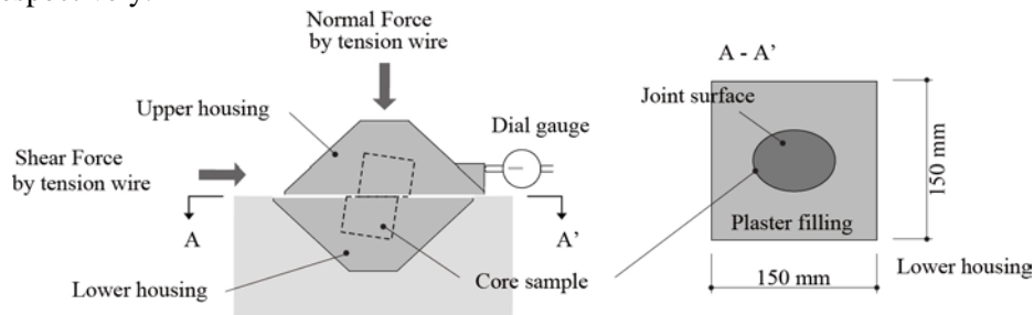
Figure 2. Setup for direct shear tests
