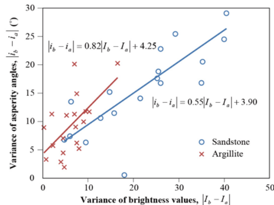
Figure 6. Correlations between variances of brightness index ( I ) and asperity angles ( i )
