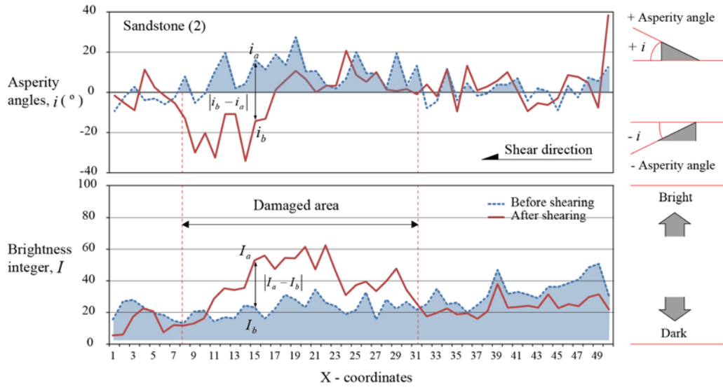
Figure 5. Brightness integers of greyscale images and asperity angles, sandstone (2)
