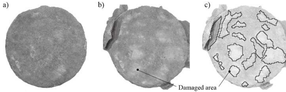
Figure 3. Greyscale images of sandstone samples before shearing (a), after shearing (b) and damaged areas determined by visual observation (c) (Sandstone (1))
