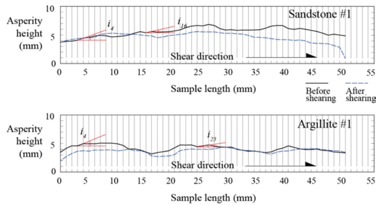
Figure 4. Joint roughness profiles of core samples measured by a profile gauge
