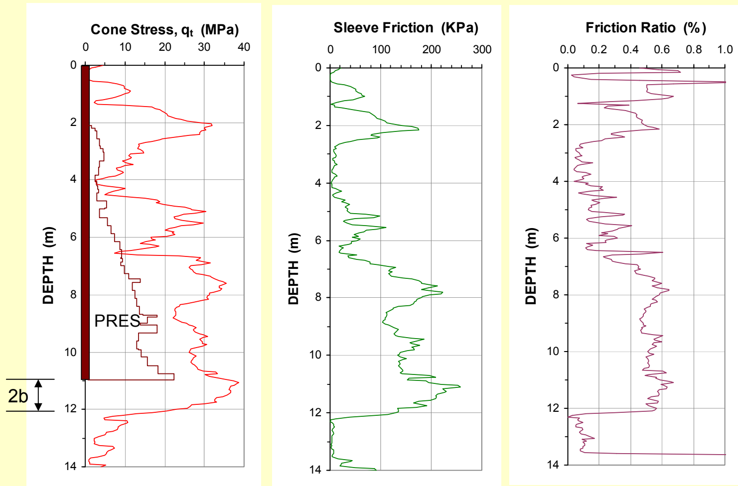
CPT sounding next to an 11 m long, 460 mm square precast concrete pile driven in silica sand in North-East Florida
