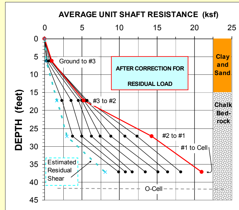
Corrected for Residual Load
