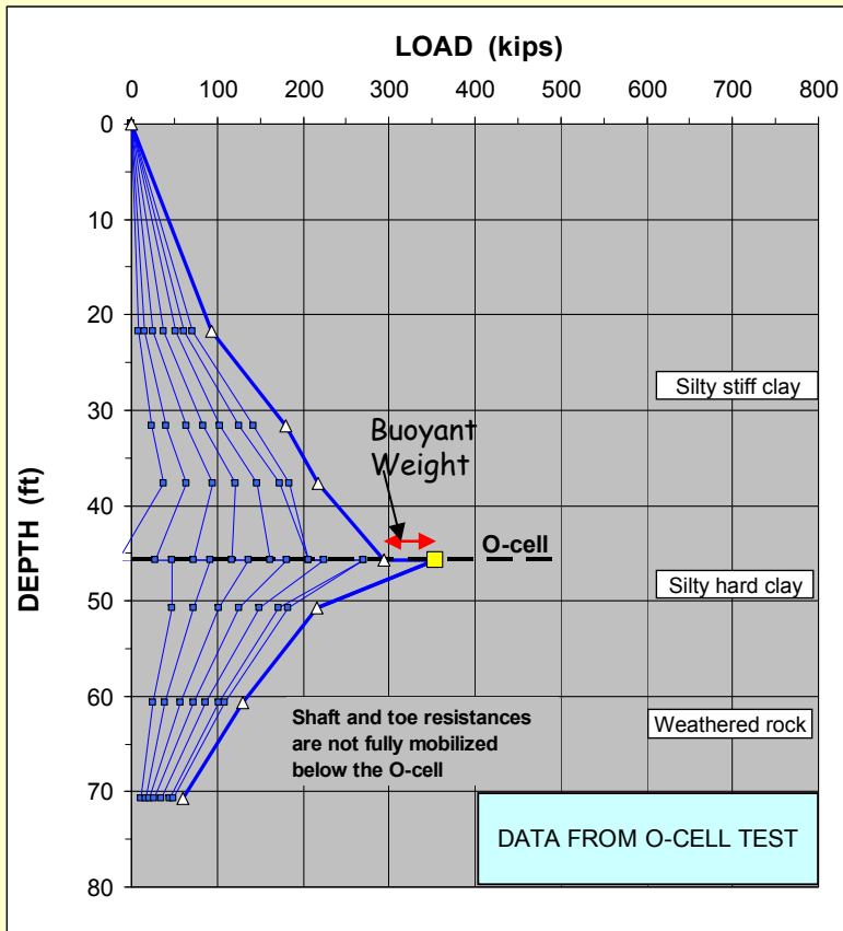
The load distribution after tangent-modulus evaluation of pile stiffness
