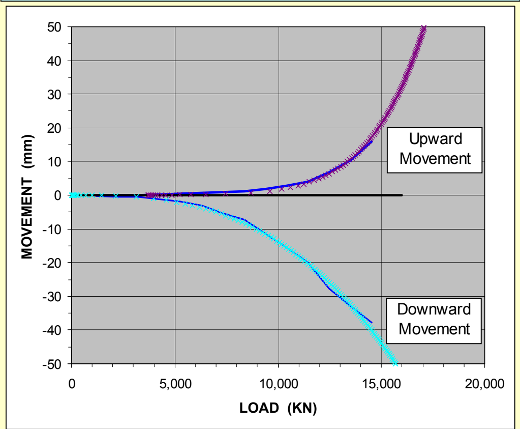
Load-Movements. Measured and Fitted to UniPile Calculation.
