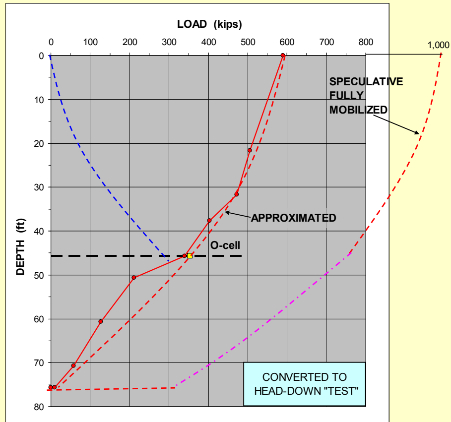
The "head-down" load distribution and speculative fully mobilized resistance
