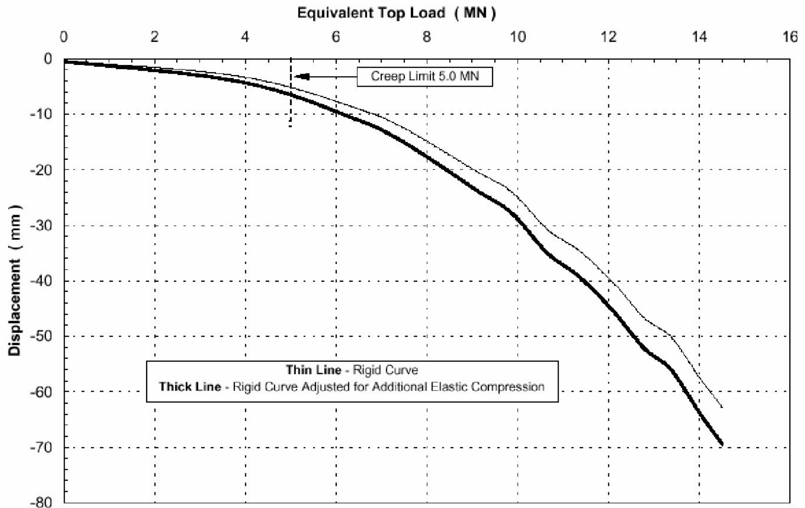
Equivalent Top Load Load-Movement Curve Test Shaft #1 - US 82 over Mississippi River - Washington Co., MS
