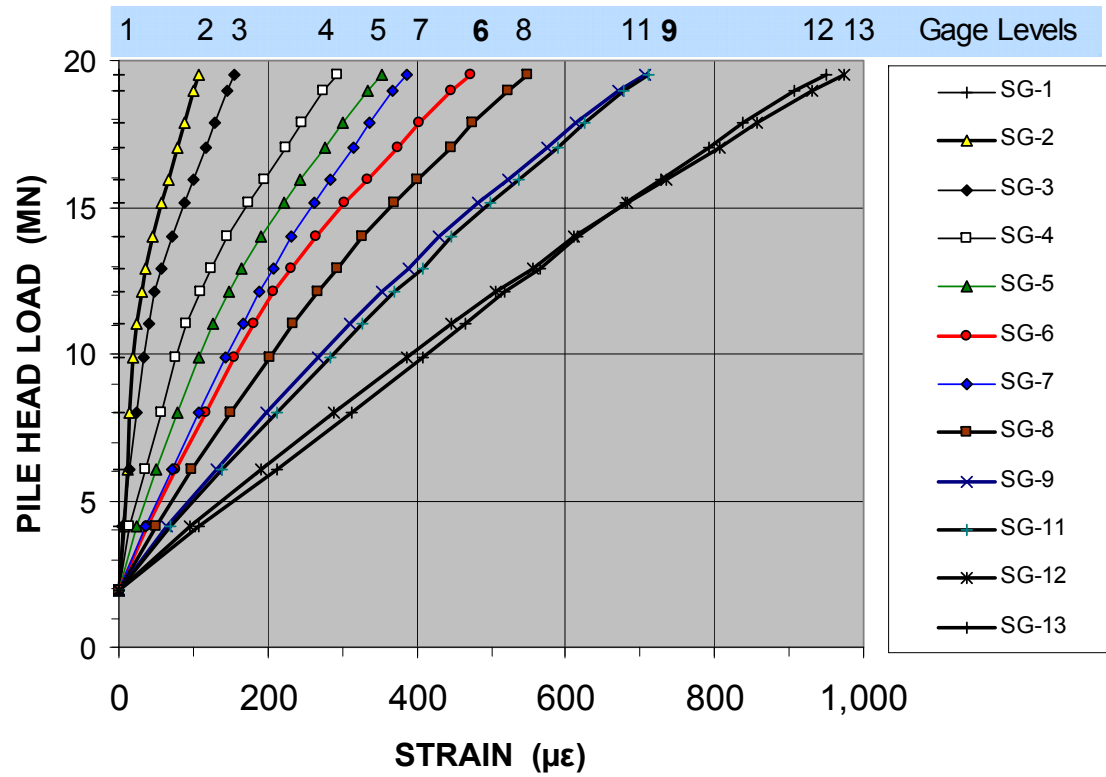
UTP-3 Load-Strain
