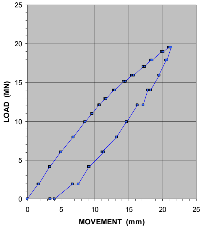
UTP-3 Load-Movement
