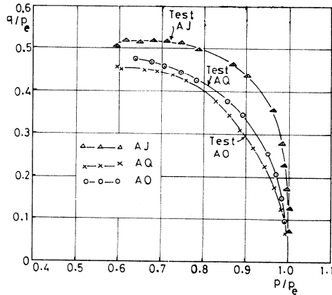
Fig. 8. State paths followed by specimens prepared under the same initial one-dimensional stress, but sheared from different isotropic stress states with constant- p stress paths.
