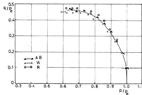
Fig. 6. State paths followed by specimens prepared under identical conditions and sheared from the same isotropic stress state with constant cell pressure and load increments but with varying load increment durations.
