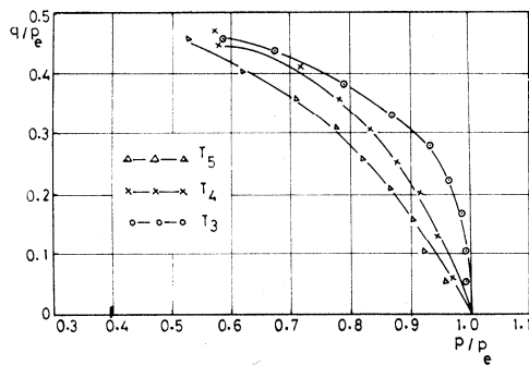
Fig. 7. State paths followed by specimens prepared under the same initial one-dimensional stress, but sheared from different isotropic stress states with constant cell pressure.
