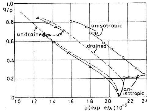
Fig. 2. State paths followed in [q/p, p \exp(e/\lambda)] space of specimens sheared along undrained, fully drained and anisotropic consolidation paths (after ROSCOE & THURAIRAJAH, 1964).
