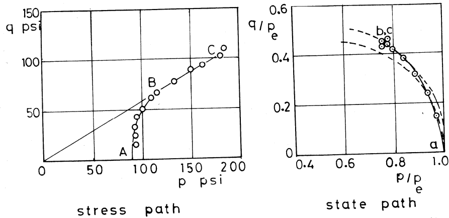
Fig. 13. Stress path and state path followed by specimen BL during anisotropic consolidation.
