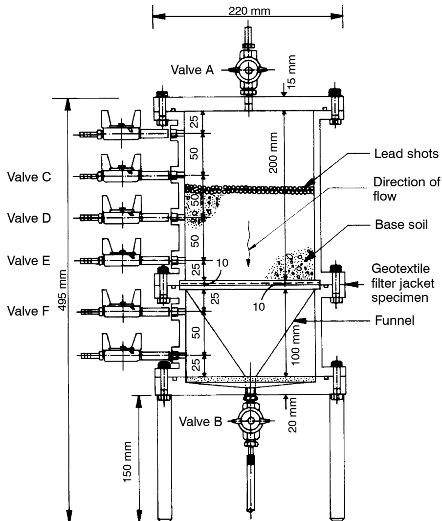
Figure 3. Filtration test apparatus.
