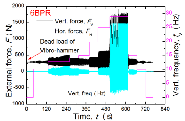
Figure 13 Time changes of input vibration frequency, f_v , vertical force, F_v , and horizontal force, F_H , in the case of 6BPR
