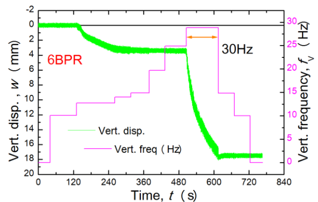
Figure 14 Time changes of input vibration frequency, f_v , and vertical displacement, w , in the case of 6BPR
