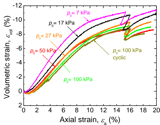
(b) Axial strain \varepsilon_a vs volumetric strain \varepsilon_{vol}
