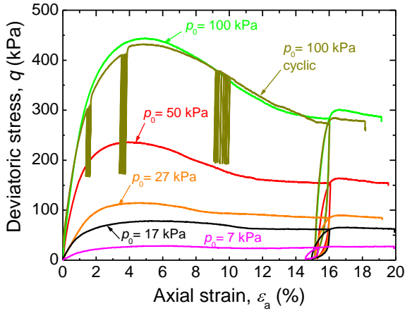
(a) Axial strain \varepsilon_a vs deviatoric stress q
