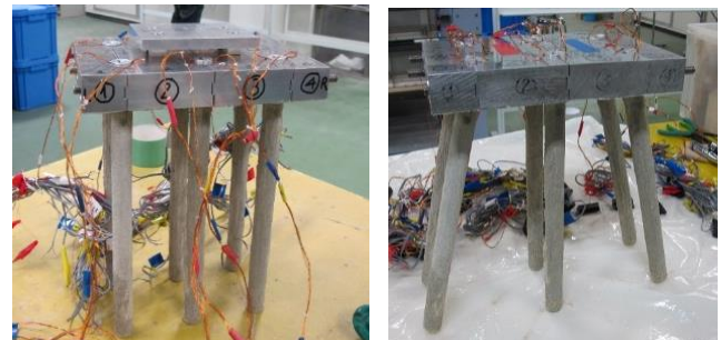
Figure 1 Pile foundation models
