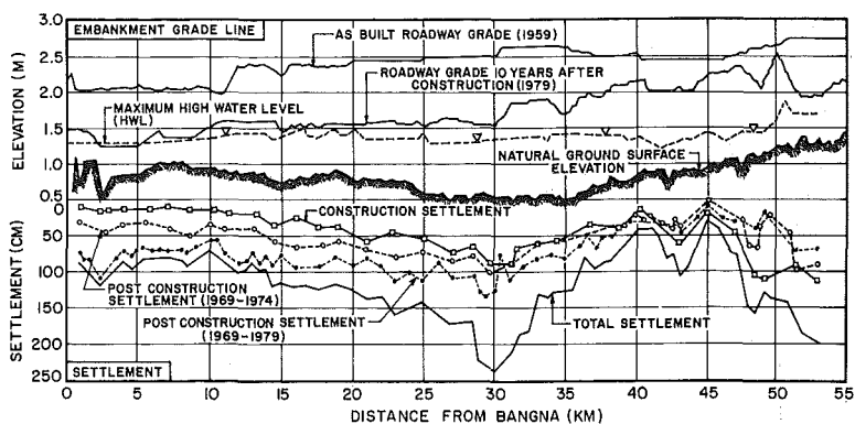
FIG. 2. Ground Elevations and Settlement Profiles (Cox 1981)
