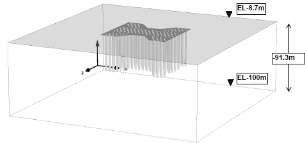
Figure 9. Schematic of PLAXIS 3D Model
