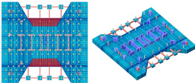
Figure 11. 3-D Finite Element Analysis Model at raft level.
