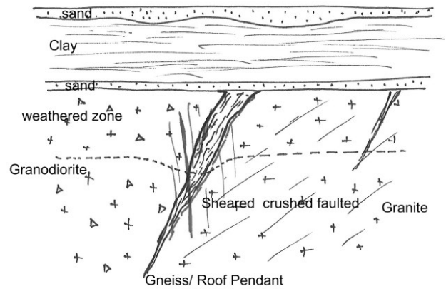
Figure 2. Diagrammatic Geological Model
