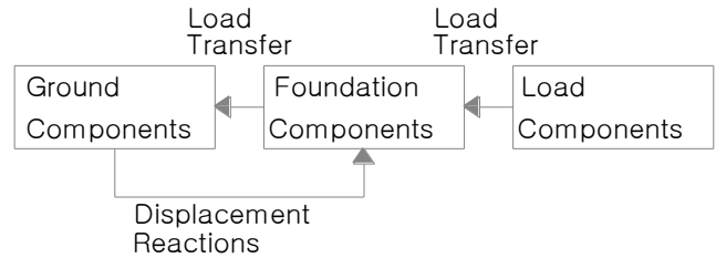
Figure 5. Main Components of Foundation Analysis
