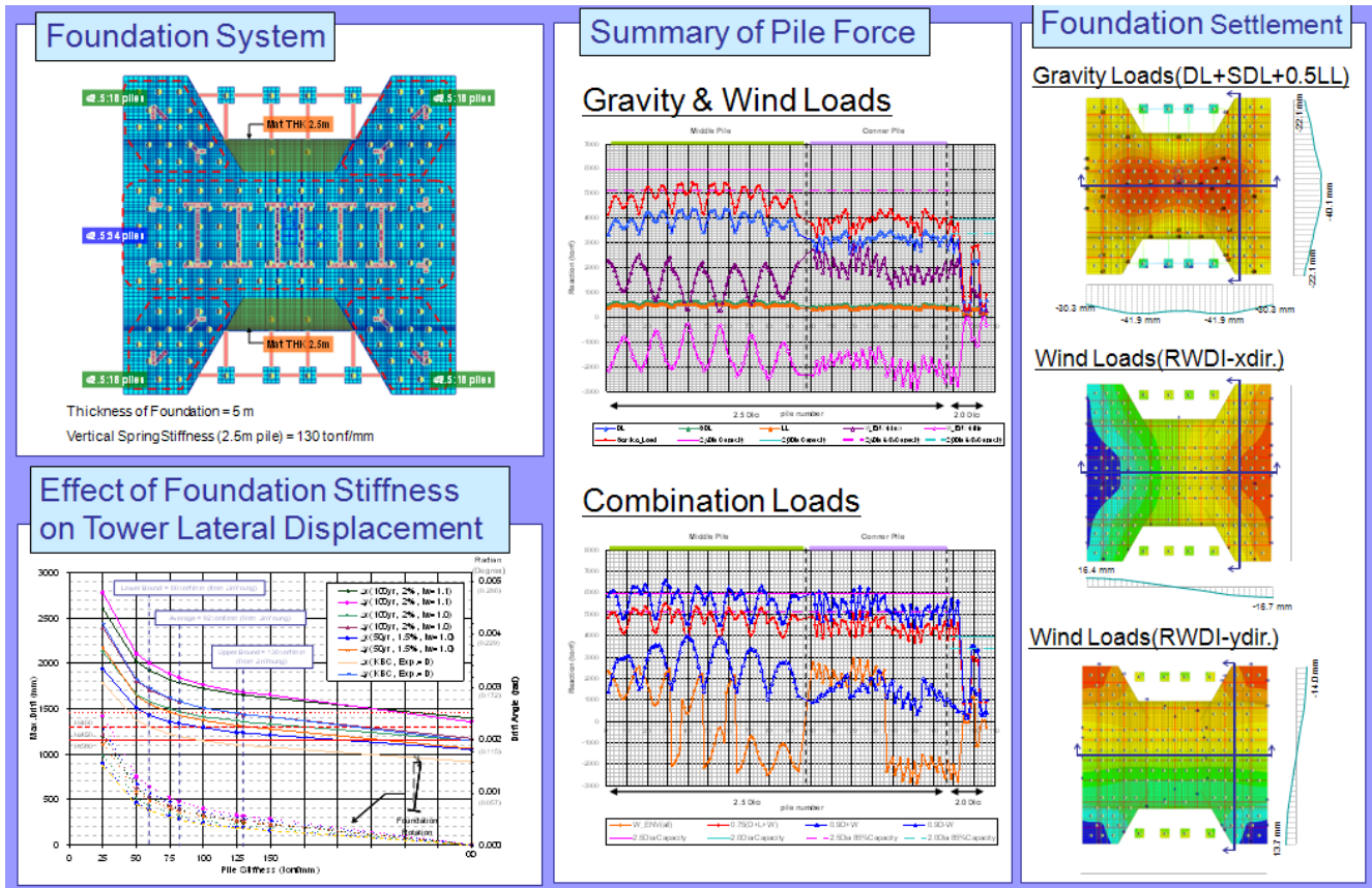
Figure 12. Summary of Foundation Analysis from Midas Program; Soil-Structure Interaction
