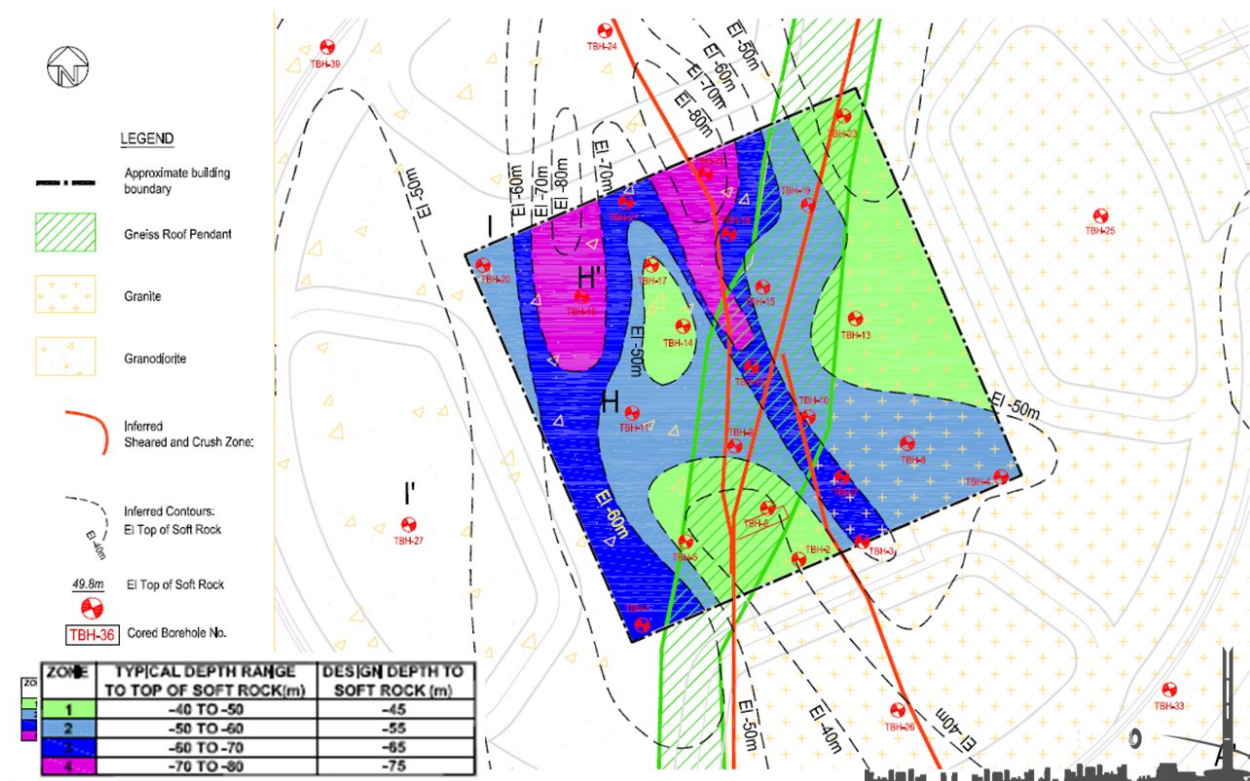
Figure 3. Inferred Contours of Top of Soft Rock
