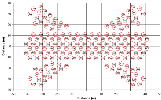
Figure 8. Computed Pile Head Vertical Stiffness Values (MN/m)
