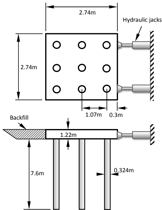
Figure 1. Lateral pile loading test layout
