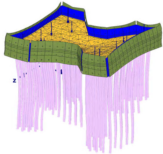
Figure 11. Deformed raft under vertical loading (Case 2).
