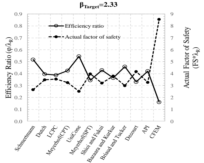
Figure 7 Efficiency ratio and actual factor of safety for different methods (Heidarie et al., 2019 a)
