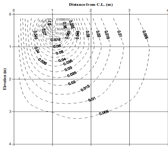
Figure 19 Contours of horizontal displacement
