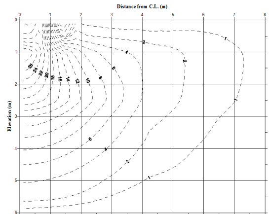
Figure 17 Contours of generated EPWP (kPa) for Drop 3 with an initial degree of saturation of 85%
