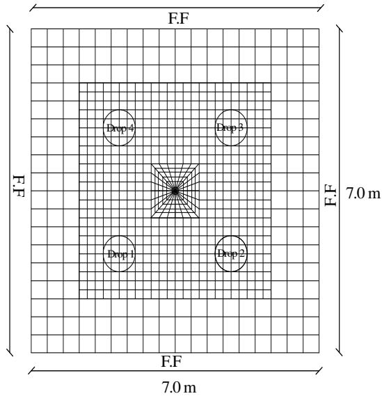
Figure 14 Top view of generated mesh
