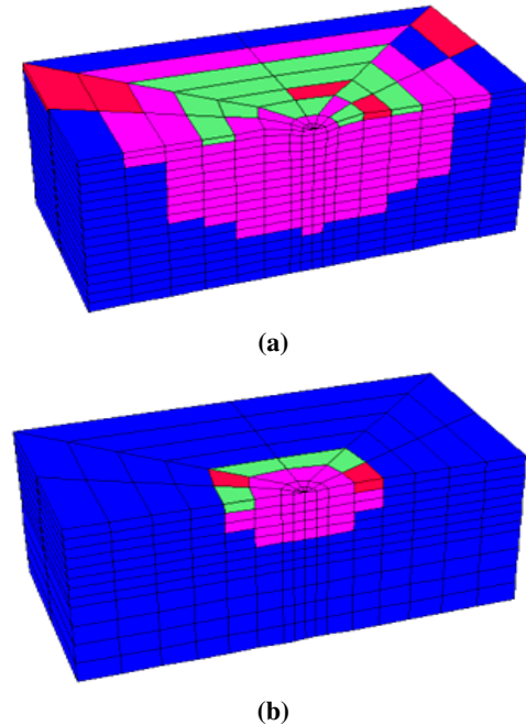
Figure 3 Finite element simulation results of stress contours under simulated load for (a) S = 100\% and (b) S = 75\%
