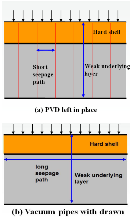
Figure 5 Comparison of drainage path: (a) PVD left in place and (b) vacuum pipes withdrawn
