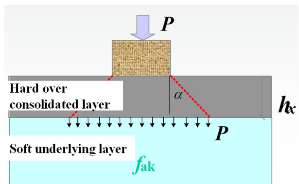
Figure 4 Effective stress distribution due to hard, over consolidated top clay layer
