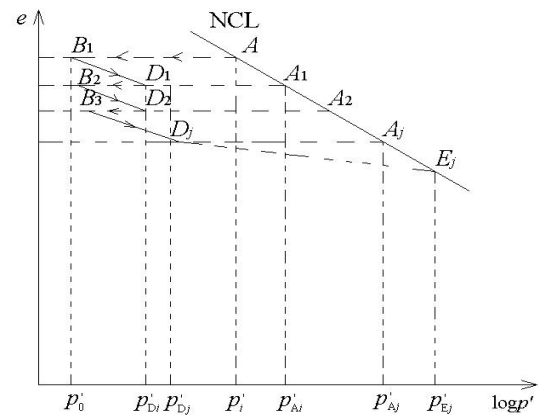
Figure 6 An e - \log p' plot showing multiple cycles of dynamic impact and vacuum consolidation
