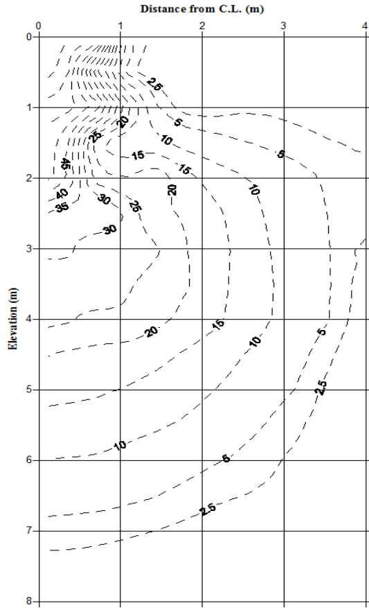
Figure 18 Contours of total vertical stress
