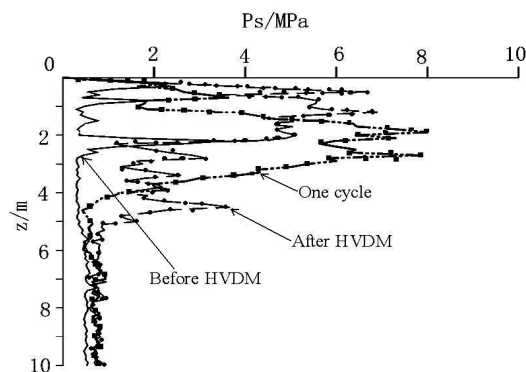
Figure 8 CPT cone resistance readings before and after ground improvement
