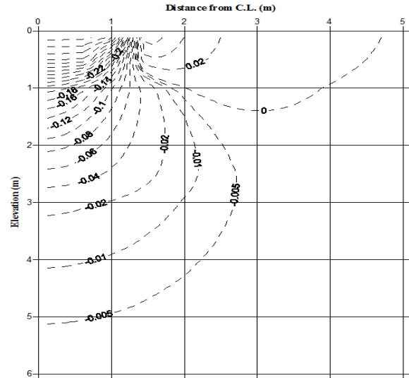
Figure 20 Contours of vertical displacement
