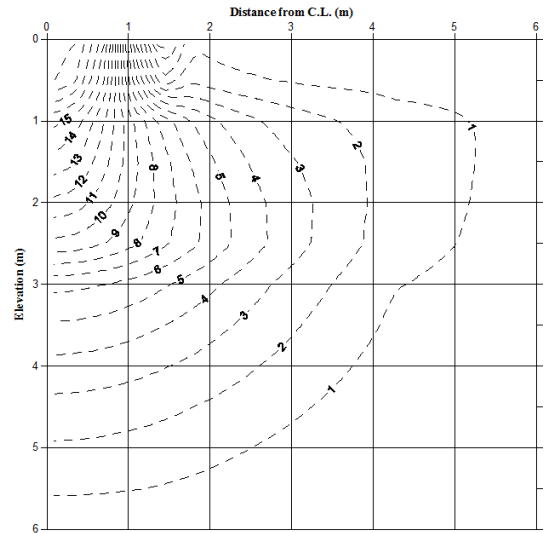
Figure 16 Contours of generated EPWP (kPa) for Drop 1, with an initial degree of saturation of 85%
