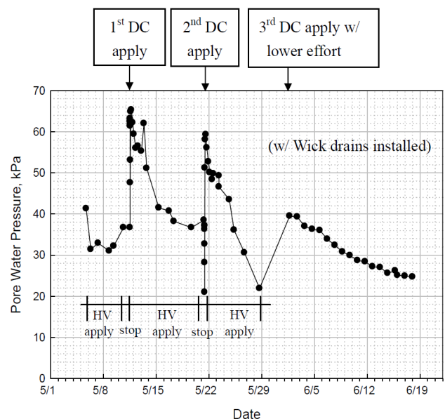
Figure 9 Pore pressure response with vacuum pipes and PVDs
