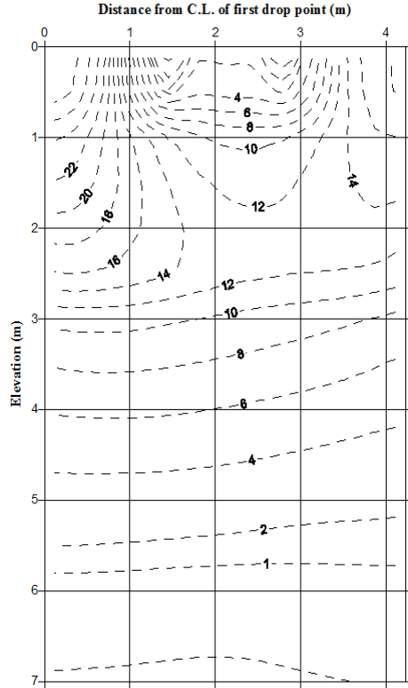
Figure 15 Contour of generated EPWP after finishing all drops around vacuum pipe
