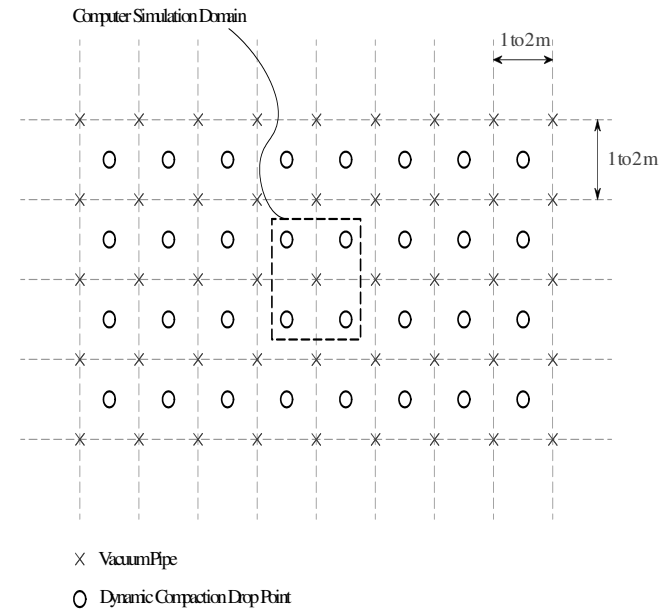
Figure 13 General pattern of HVDM
