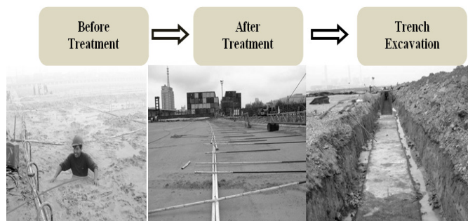
Figure 7 Photos of site conditions at Ningbo Port before and after ground improvement
