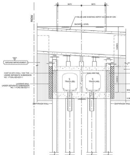
Figure 15 Underpinning work at Depot Access crossing
