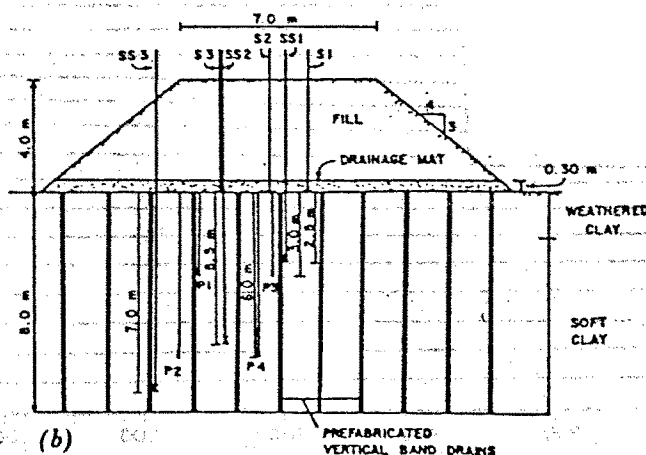
FIG. 4. Embankment Plan, Section View, and Layout of Field Instrumentation at PVD Site
