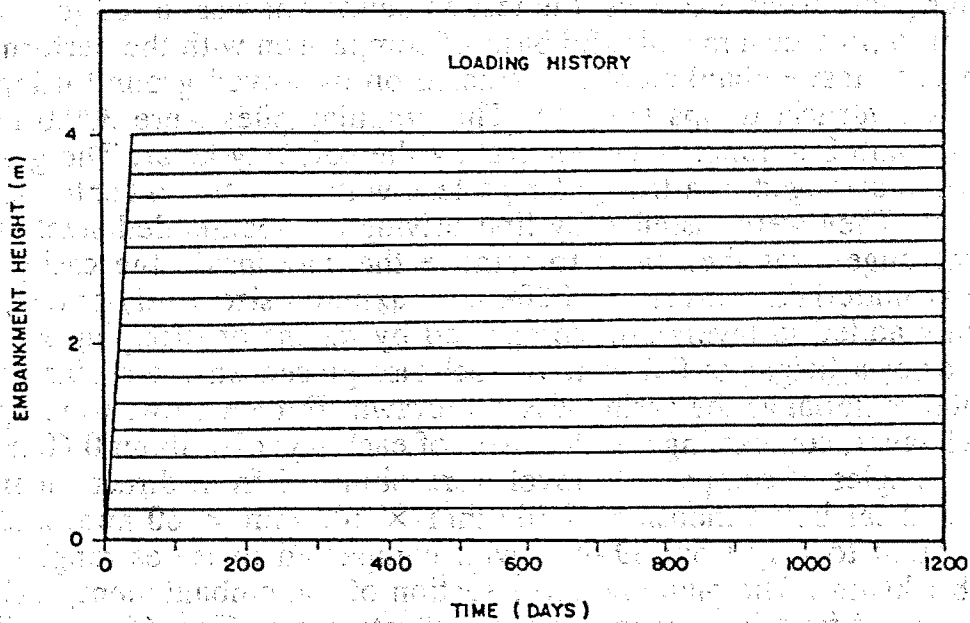
FIG. 3. Embankment Loading History at PVD Site
