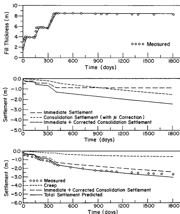
Fig. 10. Comparison of predicted settlements with observations after incorporating creep
