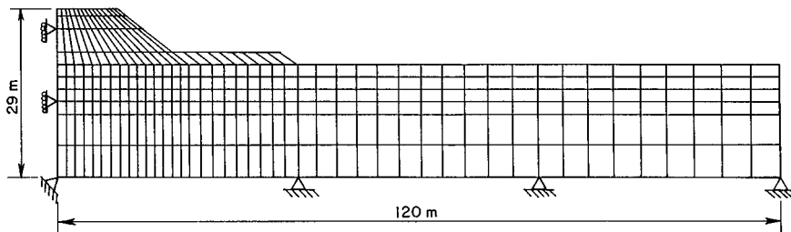
Fig. 7. Finite element mesh for embankment stabilized with sand compaction piles
