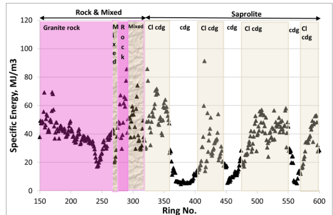
Figure 12 The Specific Energy for Tunnel A, Rings 150 to 600
