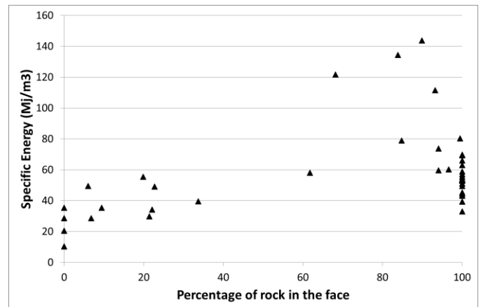
Figure 16 Specific Energy plotted against percentage of rock in the face, Tunnel B
