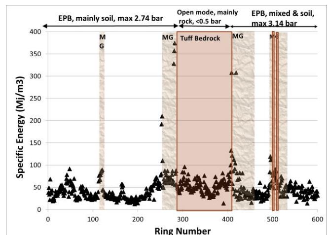
Figure 14 Specific Energy for Tunnel B, Rings 1 to 600
