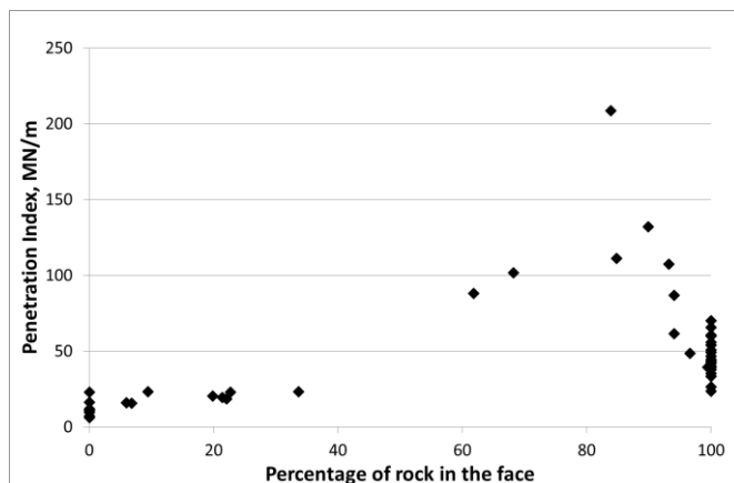
Figure 15 Penetration Index plotted against percentage of rock in the face, Tunnel B
