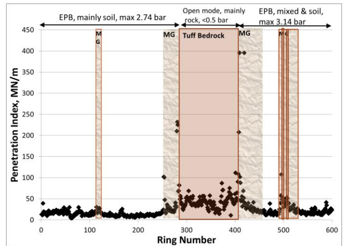
Figure 13 Penetration Index for Tunnel B, Rings 1 to 600
