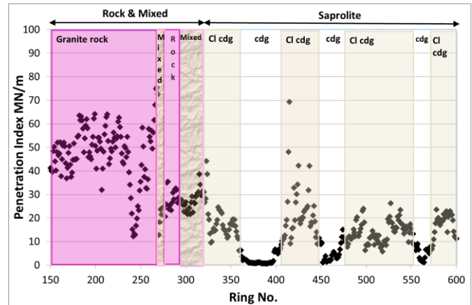
Figure 11 The Penetration Index for Tunnel A, Rings 150 to 600
