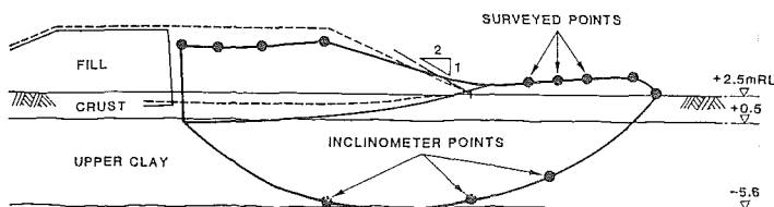
FIG. 3. Failure Mode of Embankment and Foundation (Brand and Premchitt 1989)
