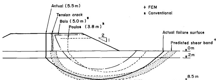
FIG. 19. Comparison of Finite-Element Predictions with Conventional Limit Equilibrium Solutions
