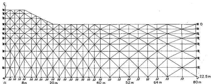
FIG. 7. Finite-Element Discretization of Embankment and Subsoils for CRISP Analysis
