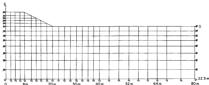
FIG. 9. Finite-Element Discretization of Embankment and Subsoils for ISBILD Analysis
