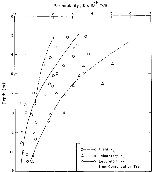
FIG. 6. Variation of Field and Laboratory Permeability with Depth
