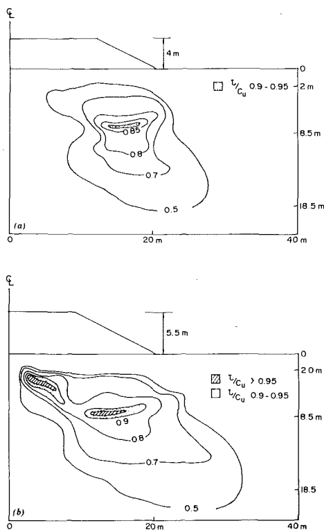
FIG. 16. Contour Plots of Normalized Shear-Stress Ratios
