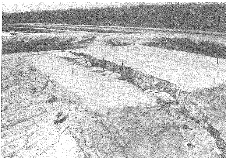
FIG. 2. View of Tensile Fracture of Compacted Fill
