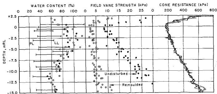
FIG. 4. Variation of Soil Properties with Depth
