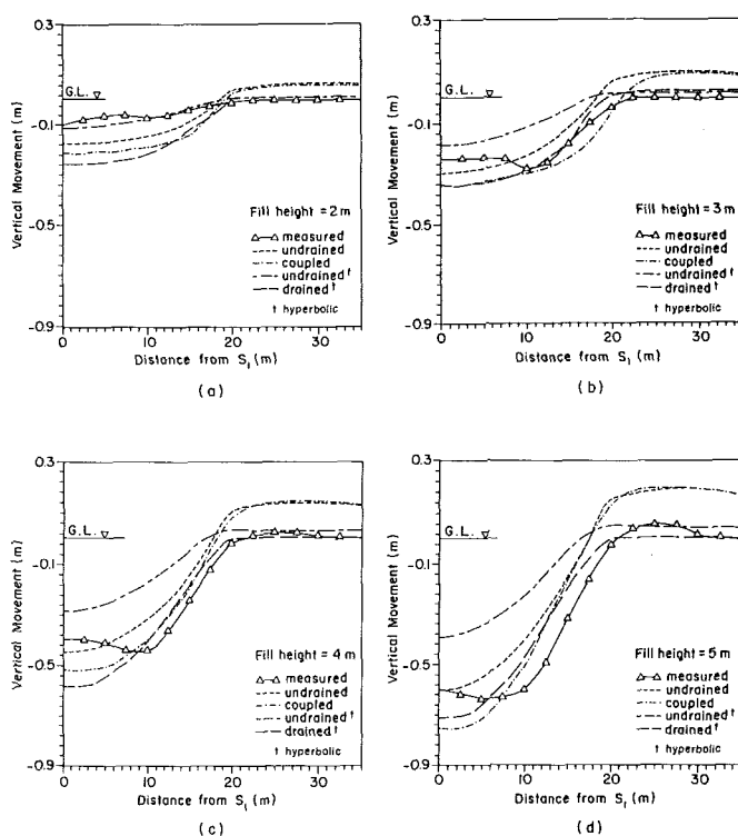
FIG. 15. Surface Settlement Profiles for Various Fill Heights
