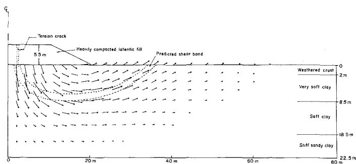
FIG. 17. Maximum Incremental Displacements at Failure
