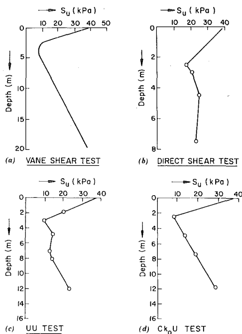
FIG. 5. Shear-Strength Profiles from Different Types of Tests
