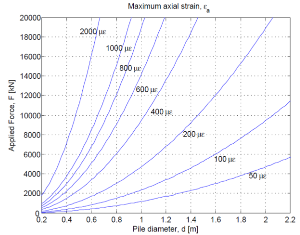
Figure 3 Maximum axial strain expected to be developed at the top of a pile during a load test, as a function of the applied load and pile diameter
