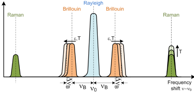
Figure 1 Components of the backscattered light spectrum in an optical fibre
