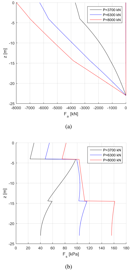
Figure 10 Profiles of computed pile response using the FE model: (a) axial pile forces, (b) shaft friction
