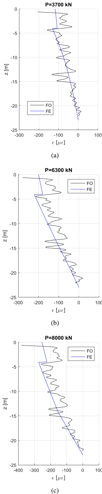
Figure 9 Profiles of observed (FO) and calculated (FE) axial strain for: (a) P=3700 kN, (b) P=6300 kN, (c) P=8000 kN
