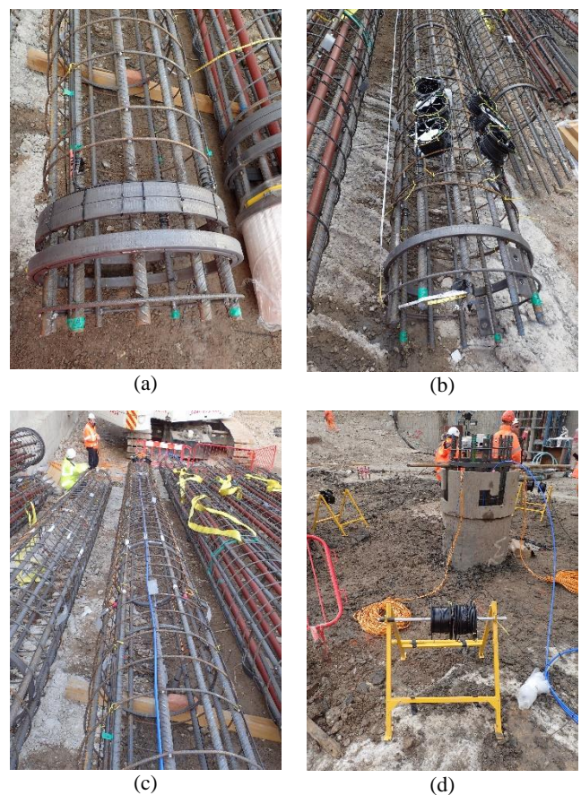
Figure 5 Stages of FO cables installation in the test pile used as a case study in Section 5: (a) FO cables anchored securely to the bottom of the bottom-most reinforcement cage, wrapped around the diameter of the cage and unreeled along the cage; (b) Remaining cables left on reels which are tied temporarily to the top of the bottom cage; (c) FO cables held to the outside of the cage by means of loose cable ties; (d) Cable reels placed on stands to be unwound as subsequent cages are lowered into the pile bore.
