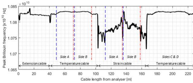
Figure 7 Baseline measurement taken from the DFOS system before the load test commenced, showing the sections of data relating to the physical location of the cables in the pile.
