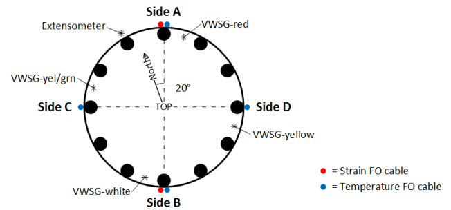
Figure 6 Cross-section of the pile cage showing the reinforcement and instrumentation positions (VWSG = vibrating wire strain gauge, FO = fibre optic).
