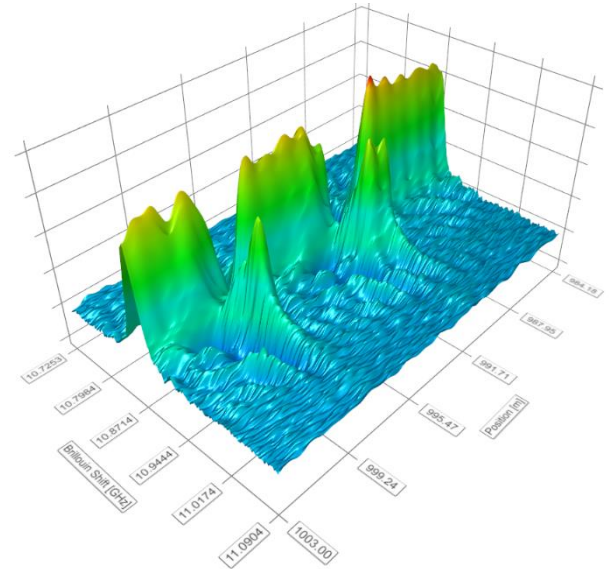
Figure 2 Three-dimensional Brillouin gain spectrum measured by Brillouin Optical Frequency Domain Analysis (fibrisTerre Systems GmbH)
