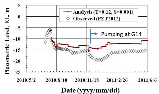
Figure 22 Comparison of observed groundwater drawdown with prediction (Yang, et al., 2012)
