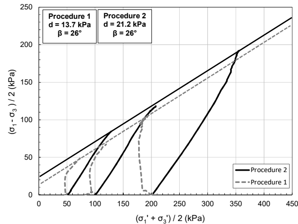
Figure 8 Point Q effective stress paths for Procedures 1 and 2
