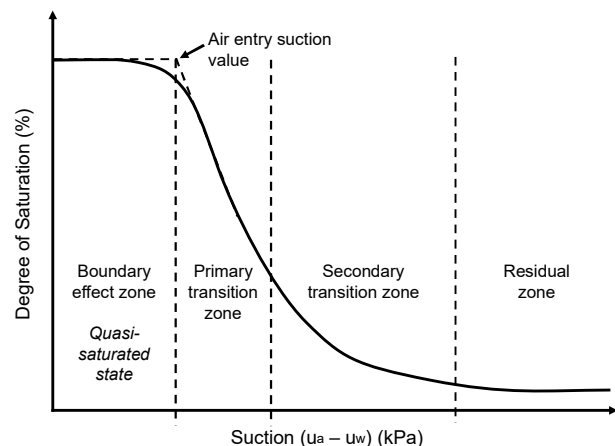
Figure 1 Desaturation zones in a hypothetical SWRC (modified from Vanapalli et al. 1996)
