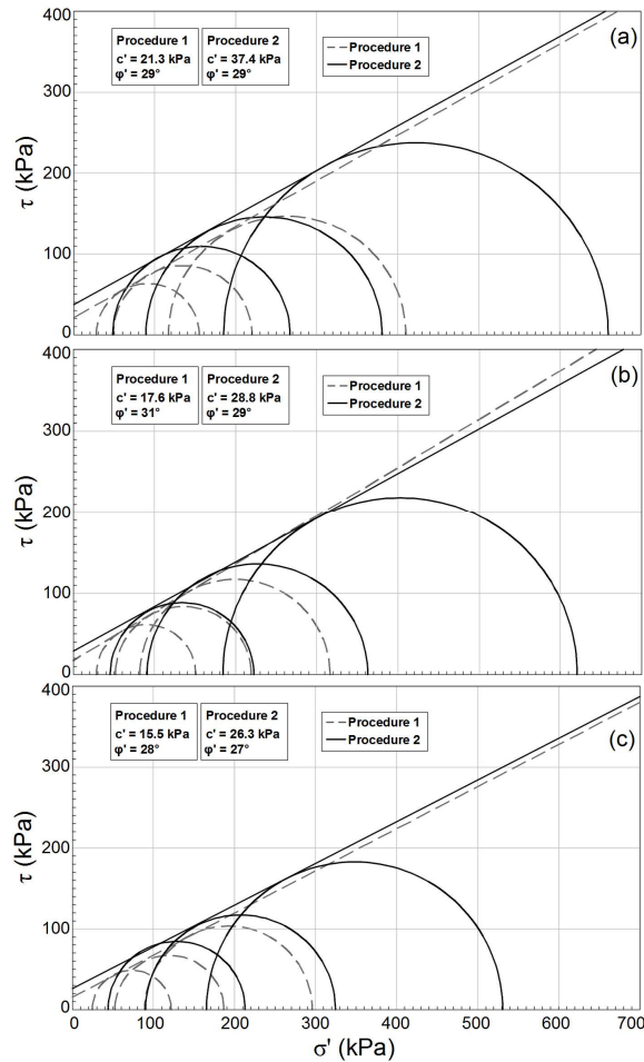
Figure 11 Mohr's circles and shear strength envelopes from Procedures 1 and 2. (a) Point O, (b) Point P, (c) Point Q
