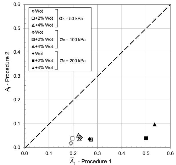
Figure 9 Parameter at failure, \bar{A}_f , obtained from the tests performed with Procedures 1 and 2
