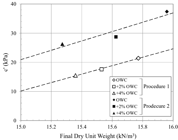
Figure 13 Effective cohesion values related to different final dry unit weight before shear for Procedures 1 and 2
