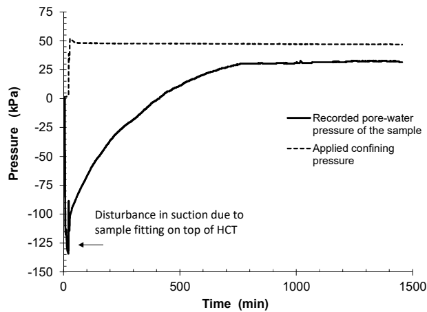
Figure 3 Suction development from a “Point O” sample during the saturation-consolidation stage in Procedure 2
