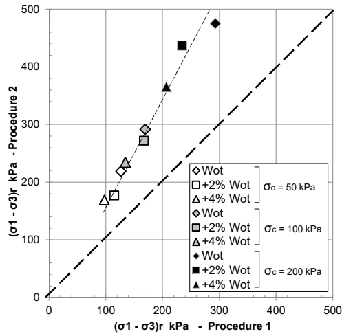
Figure 10 Deviator stresses in failure for same initial water content and consolidation conditions
