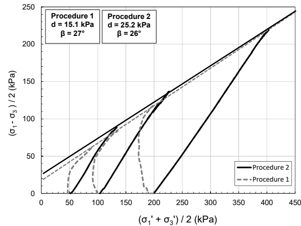
Figure 7 Point P effective stress paths for Procedures 1 and 2
