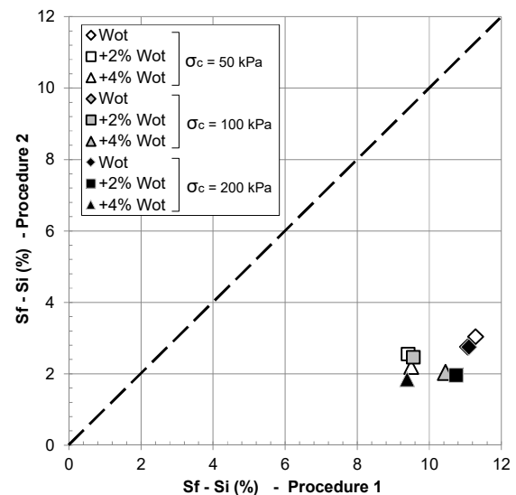
Figure 5 Difference between the final and initial degree of saturation ( S_n - S ) between Procedure 1 and 2
