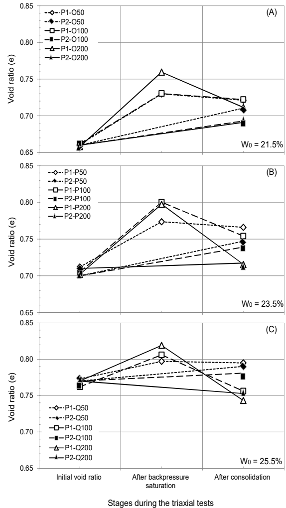
Figure 4 Void ratio variation along the triaxial tests stages for Procedures 1 and 2. (a) Point O, (b) Point P, (c) Point Q
