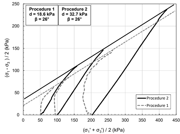
Figure 6 Point O effective stress paths for Procedures 1 and 2
