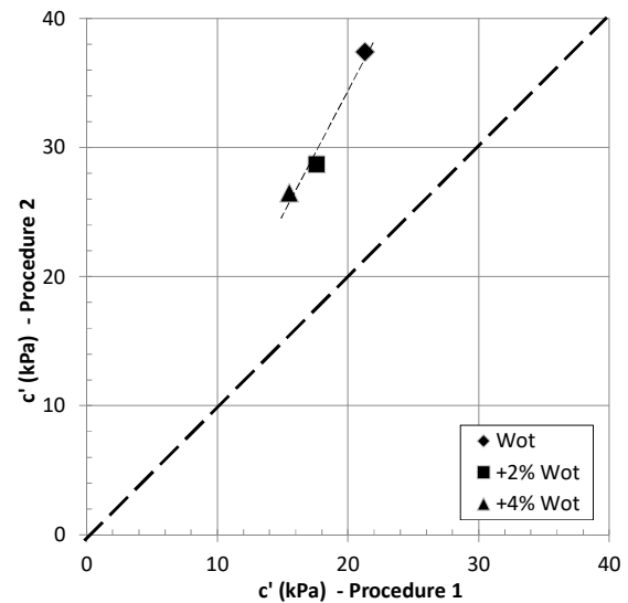
Figure 12 Effective cohesion for same initial water content and consolidation conditions
