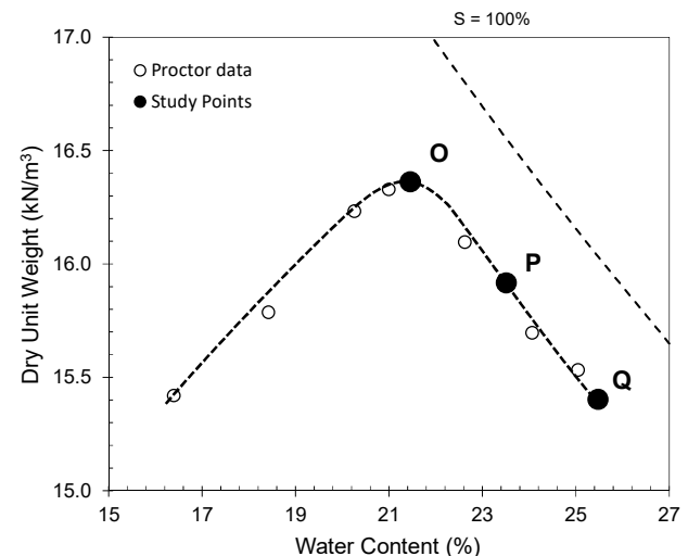
Figure 2 Compaction curve and study points O, P and Q, located at the OWC, +2%OWC and +4%OWC, respectively
