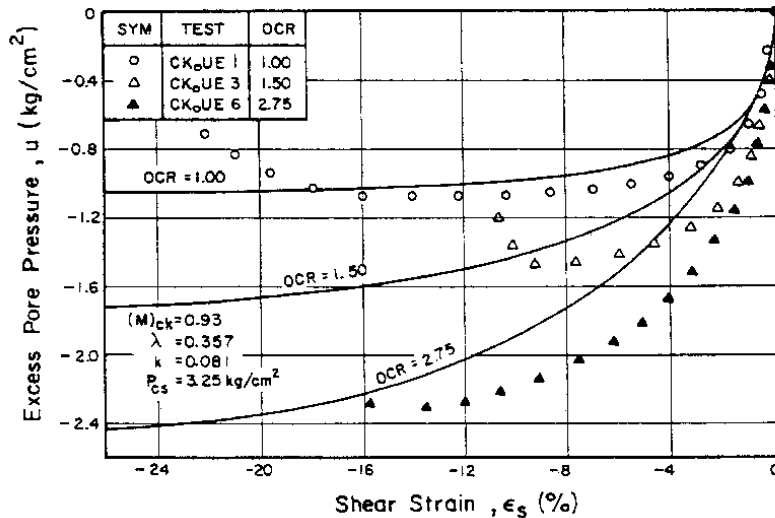
Fig. 17 ( u, \epsilon_s ) Plot for K_0 -overconsolidated Samples in Extension Conditions Compared with the Predictions from Pender's Model
