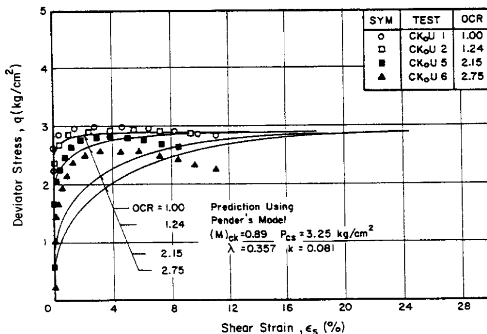
Fig. 13 ( q, \epsilon_s ) Plot for K_0 -overconsolidated Samples Compared with the Predictions from Pender's Model (Critical State)
