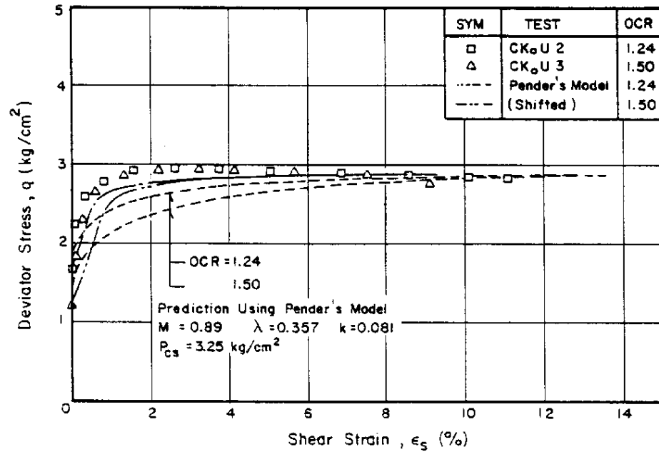
Fig. 35 ( q, \epsilon_s ) Plot for K_0 -overconsolidated Samples Compared with the Predictions from Pender's Model with and without Shifted Initial Stress Points (Wet Zone)
