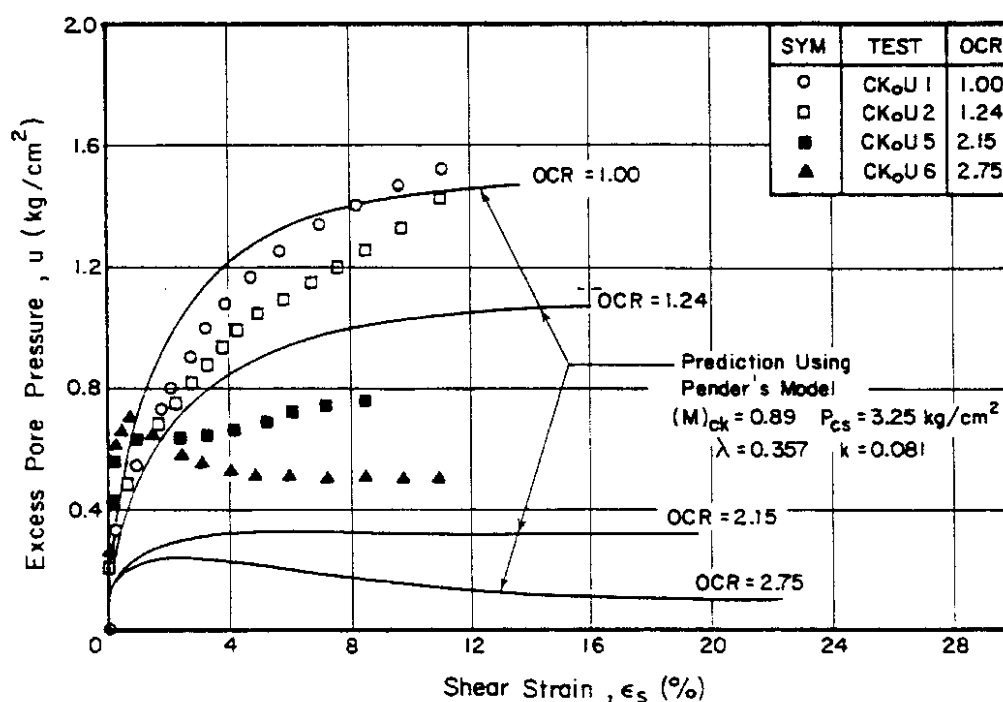
Fig. 14 ( u, \epsilon_s ) Plot for K_0 -overconsolidated Samples Compared with the Predictions from Pender's Model (Critical State)
