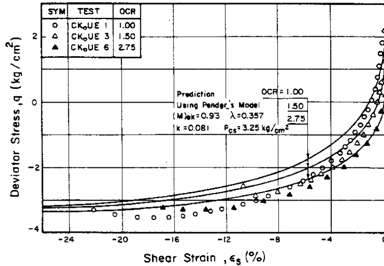
Fig. 16 ( q, \epsilon_s ) Plot for K_0 -overconsolidated Samples in Extension Conditions Compared with the Predictions from Pender's Model
