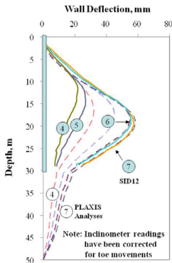
Figure 13 Comparison of results of PLAXIS analyses with inclinometer readings (Hwang, et al., 2012)
