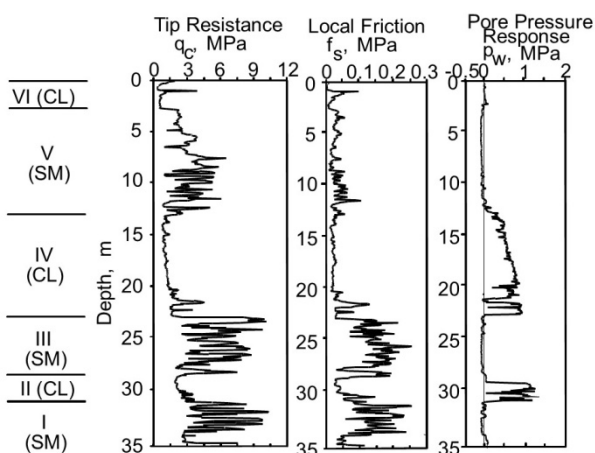
Figure 4 Typical results of cone penetration tests in T2 Zone
