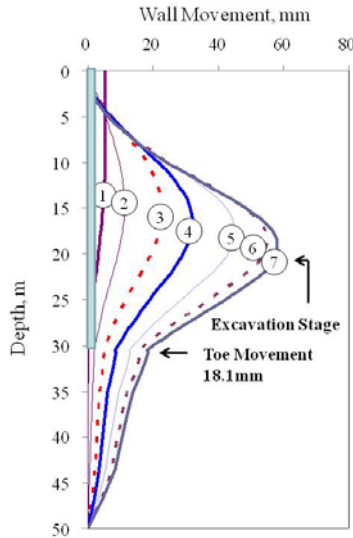
Figure 12 Wall deflection profiles obtained by PLAXIS analyses (Hwang, et al., 2012)
