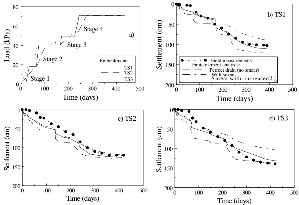
Figure 4. a) Construction loading history and (b, c and d) Surface settlement at the centre-line for embankments (b) TS1, (c) TS2 and (d) TS3, respectively, SBIA (Indraratna and Redana, 1998b).
