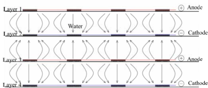
Figure 6 Use of electro-osmosis together with HDeGs
