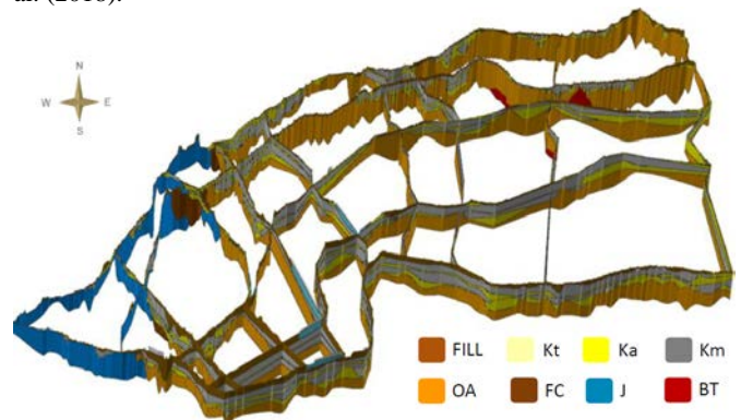
Figure 1 Fence diagram for one area in Singapore
