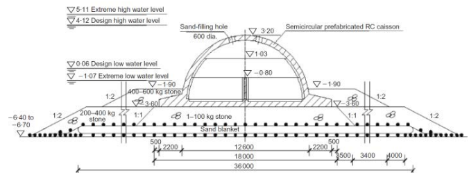
Figure 8 Use of PVDs (not shown) and the weight of the rubble mound to consolidate the soft seabed soil (not shown) before semicircular concrete caissons were placed to form a breakwater in China (after Yan et al. 2009).
