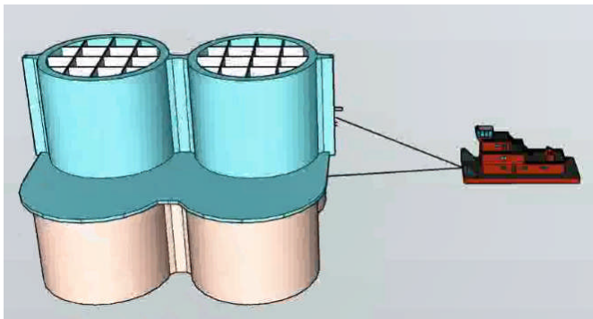
Figure 12 Towing of suction caissons with seawall structures into the seawall site for installation
