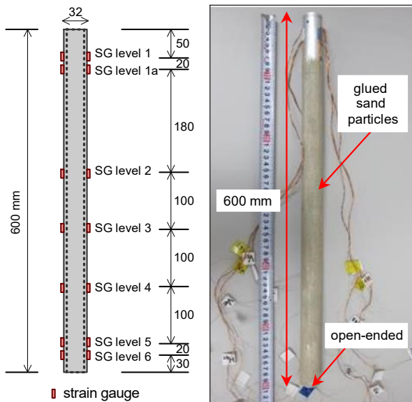
Figure 6 Configurations of the model pile for single pile load tests
