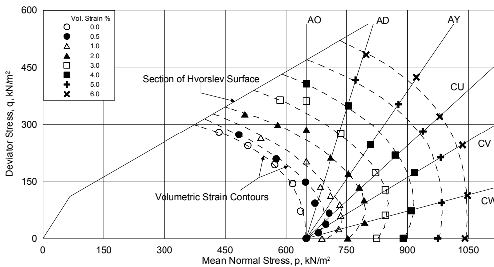
Fig. 1 Constant volumetric strain contours in (p, q) plot (Balasubramaniam, 1969)
