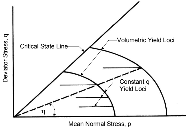
Fig. 2 Constant q yield loci
