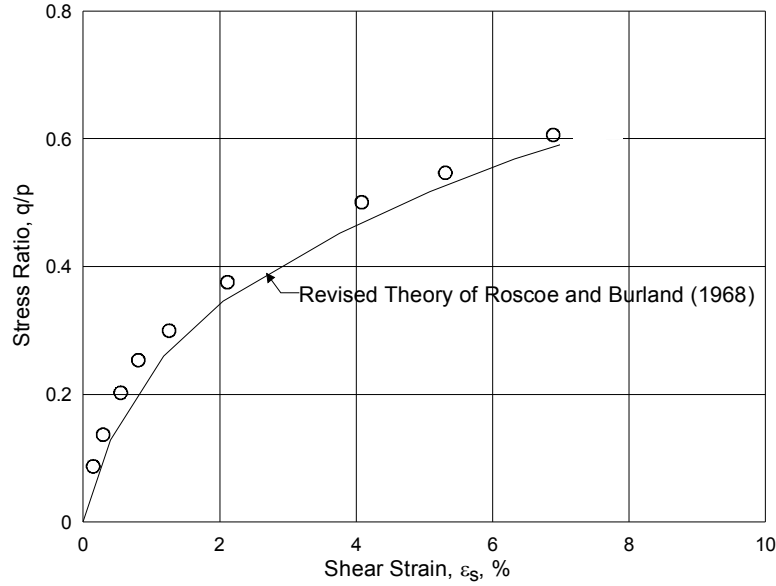
Fig. 8 Predicted shear strain by Roscoe and Burland (1968) after using contribution from constant q yield loci (Balasubramaniam, 1969)
