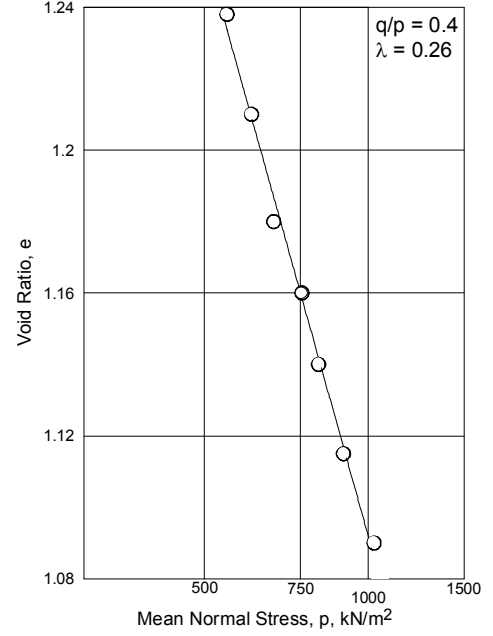
Fig. 5 Voids ratio-mean normal stress relation during isotropic and anisotropic consolidation (typical case for \eta=0.4 ) (Balasubramaniam 1969)
