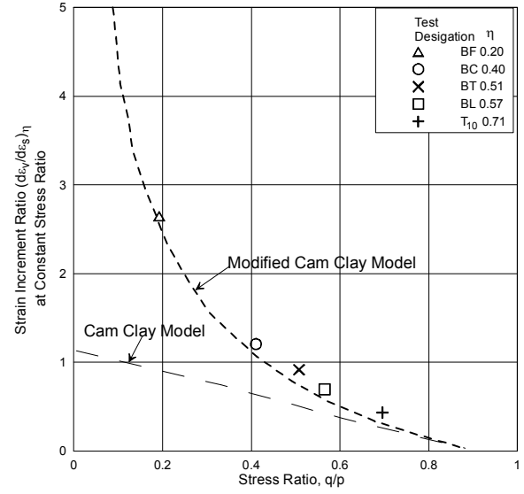
Fig. 4 Observed and predicted dilatancy ratio (Balasubramaniam, 1969)
