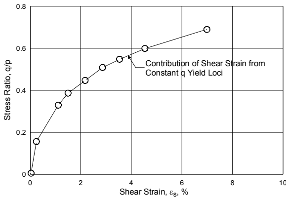
Fig. 3 Shear strain from constant q yield loci (virtually same as undrained shear strain) (Balasubramaniam, 1969)
