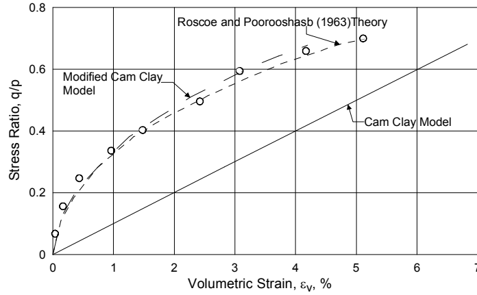
Fig. 6 Volumetric strains in constant p tests (Balasubramaniam, 1969)
