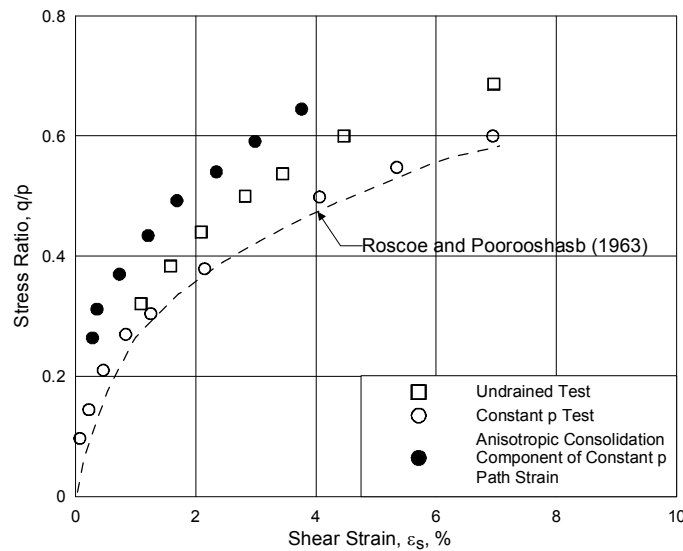
Fig. 7 Various components of shear strain (undrained, anisotropic and drained) (Balasubramaniam, 1969)
