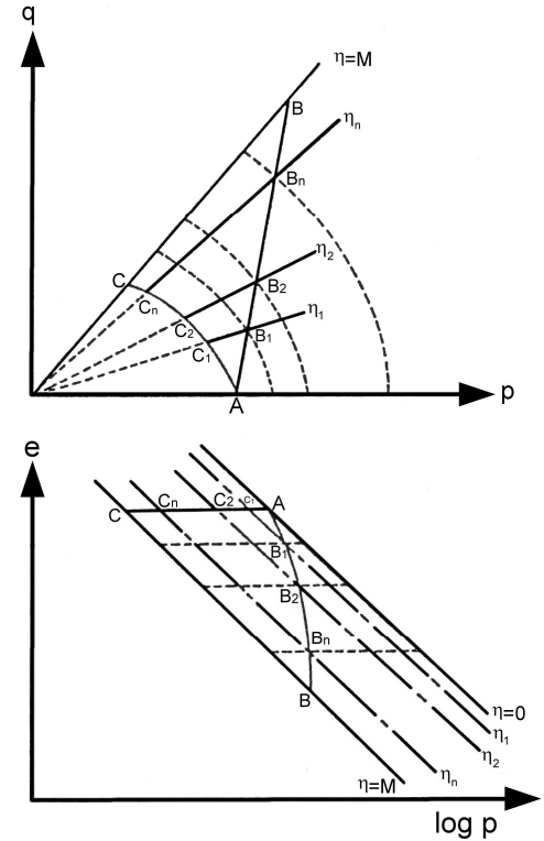
Fig. B1 Incremental steps in the calculation of volumetric and shear strains in drained tests
