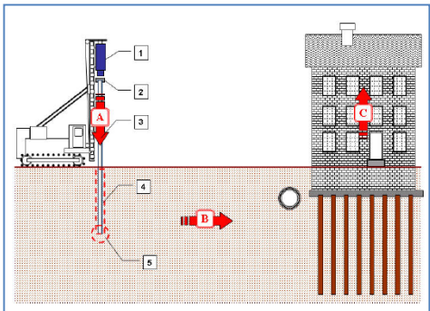
Propagation of stress wave from impact hammer (After Massarsch and Fellenius 2015)
