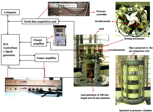
Photo 2 Resonant column apparatus (After Kumar and Cherian, 2015)
