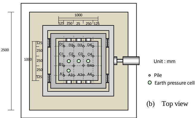
Model Pile Testing Setup (after Hamada et al. 2015)
