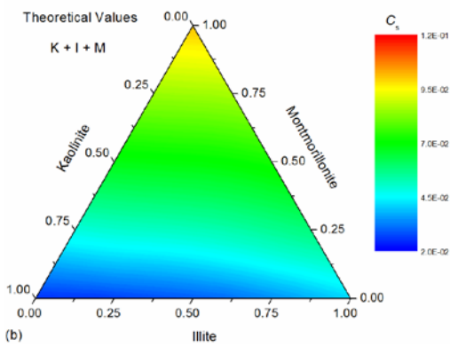
(b) Swelling index
