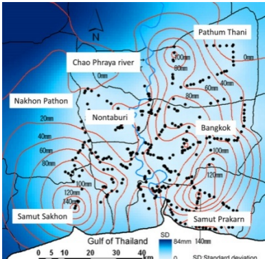
Contour lines of land subsidence in Chao Phraya Delta (After Yasuhara, Murakami and Mimura 2015)
